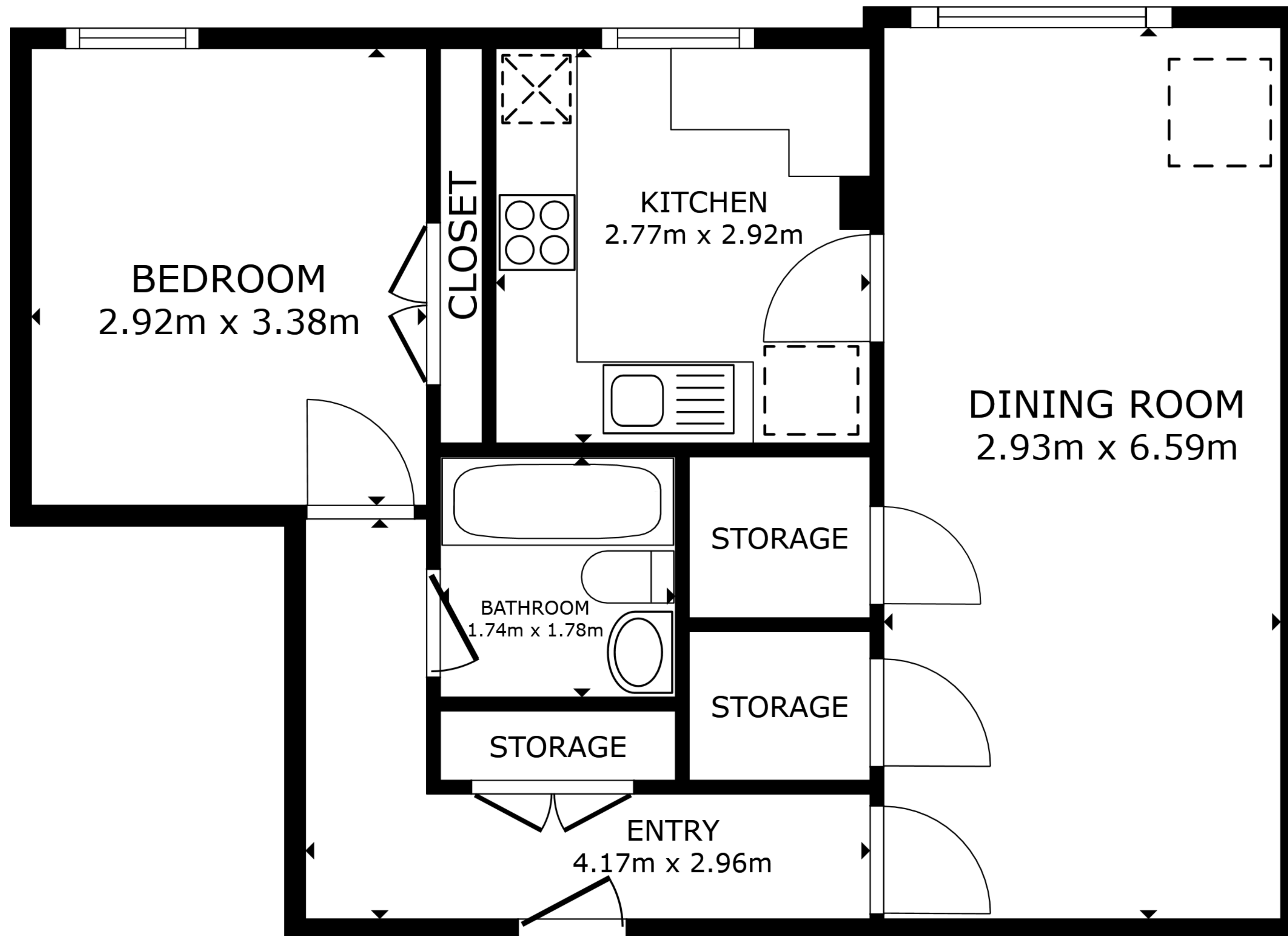
FLOOR PLAN
