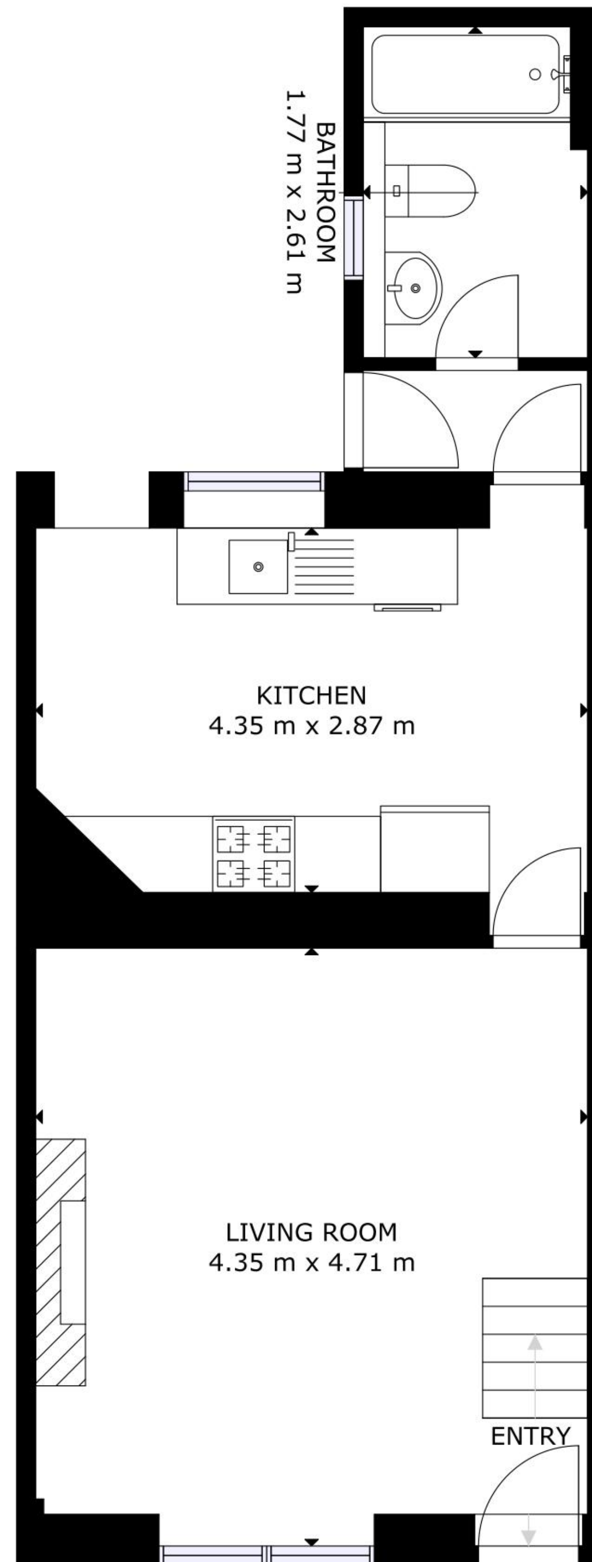
FLOOR 1
