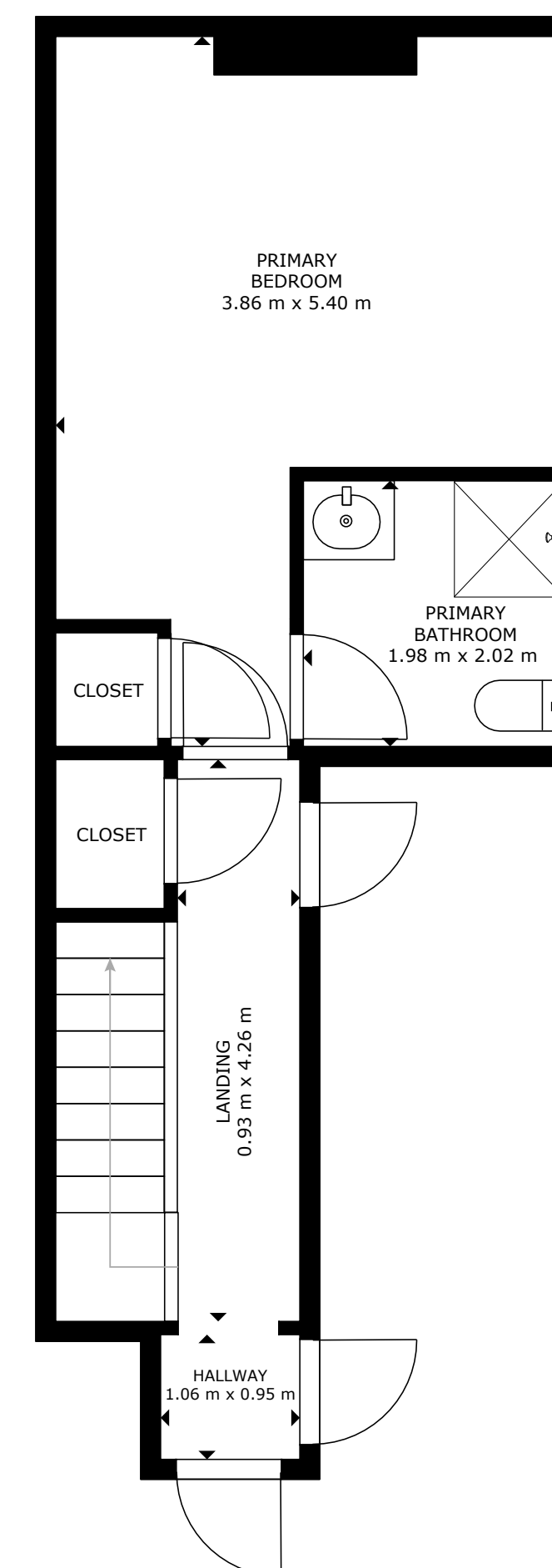
FLOOR 2
