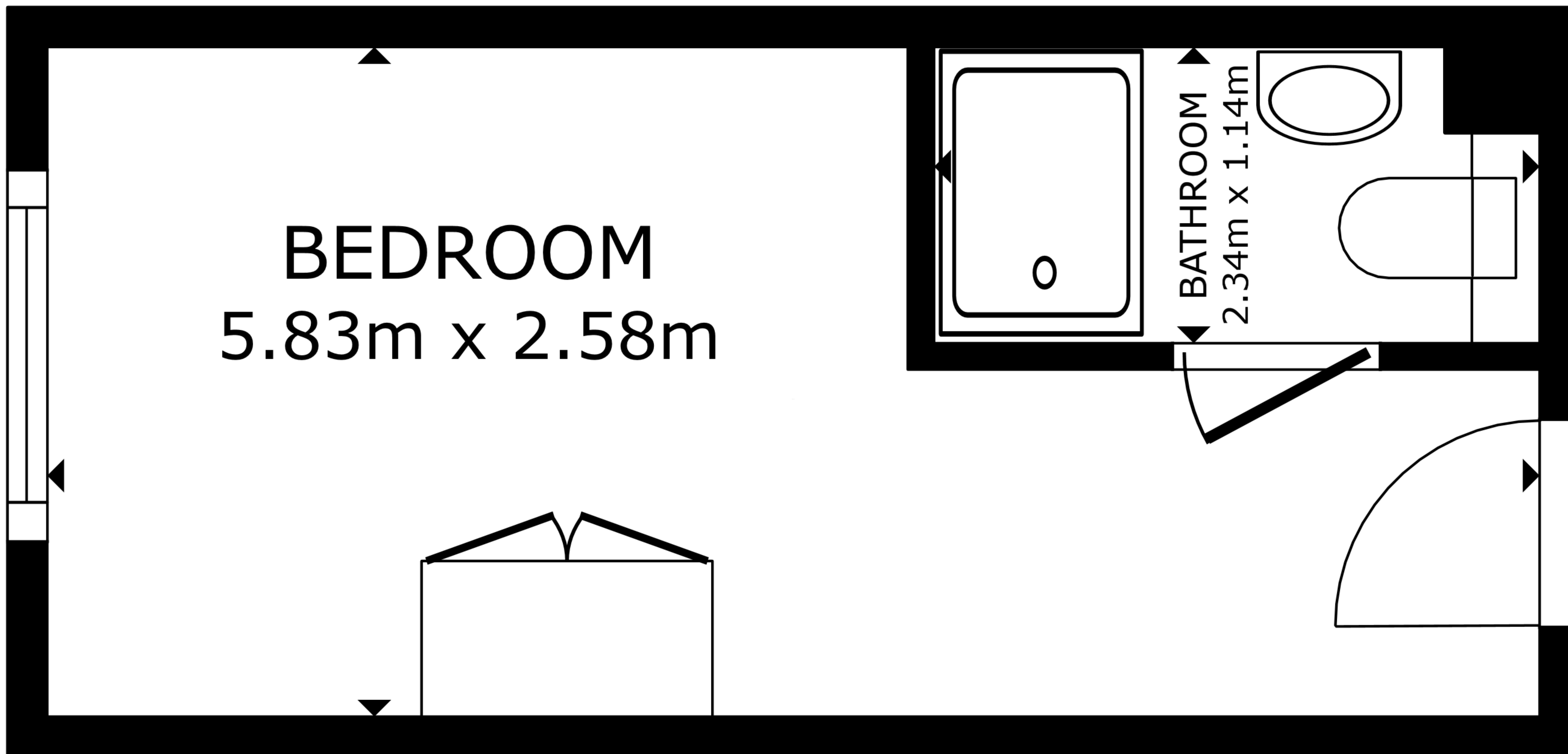
FLOOR PLAN
