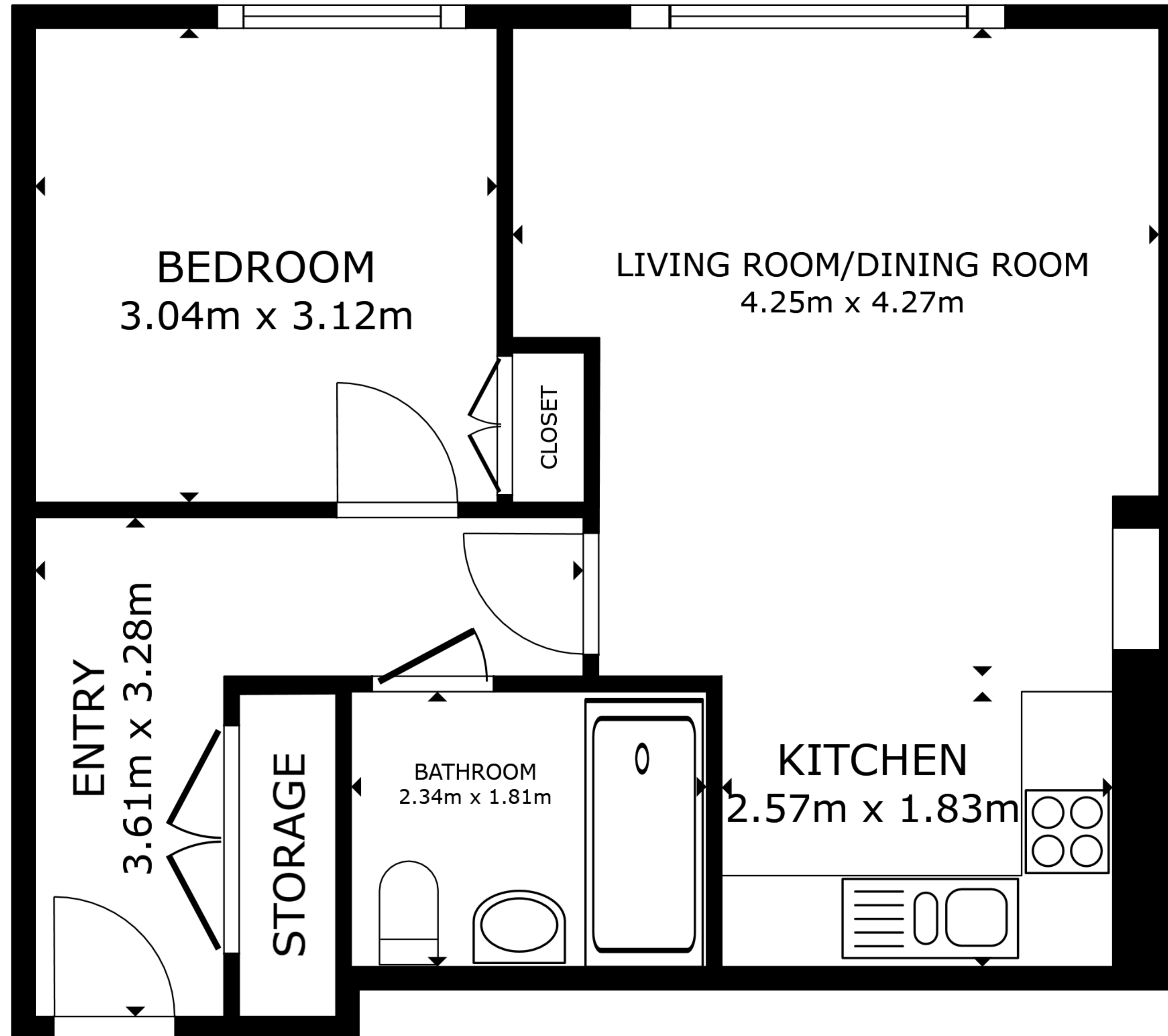
FLOOR PLAN
