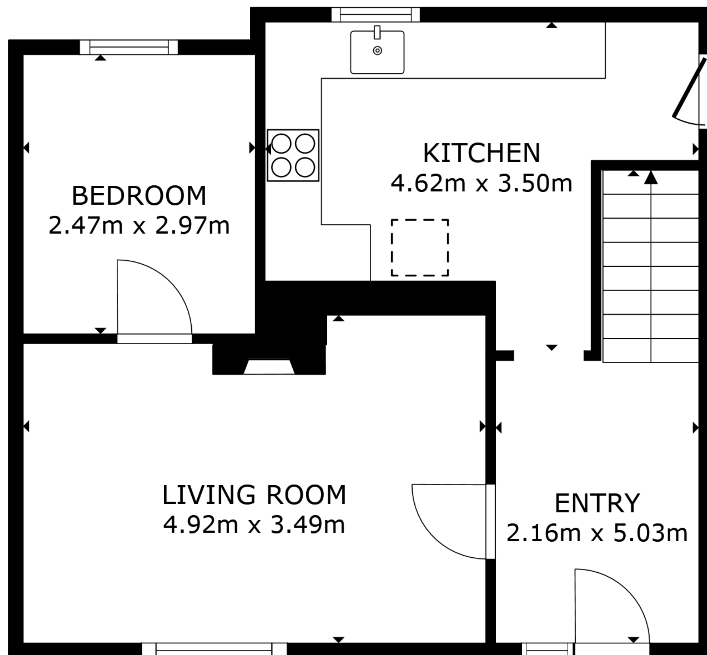
FLOOR 1
