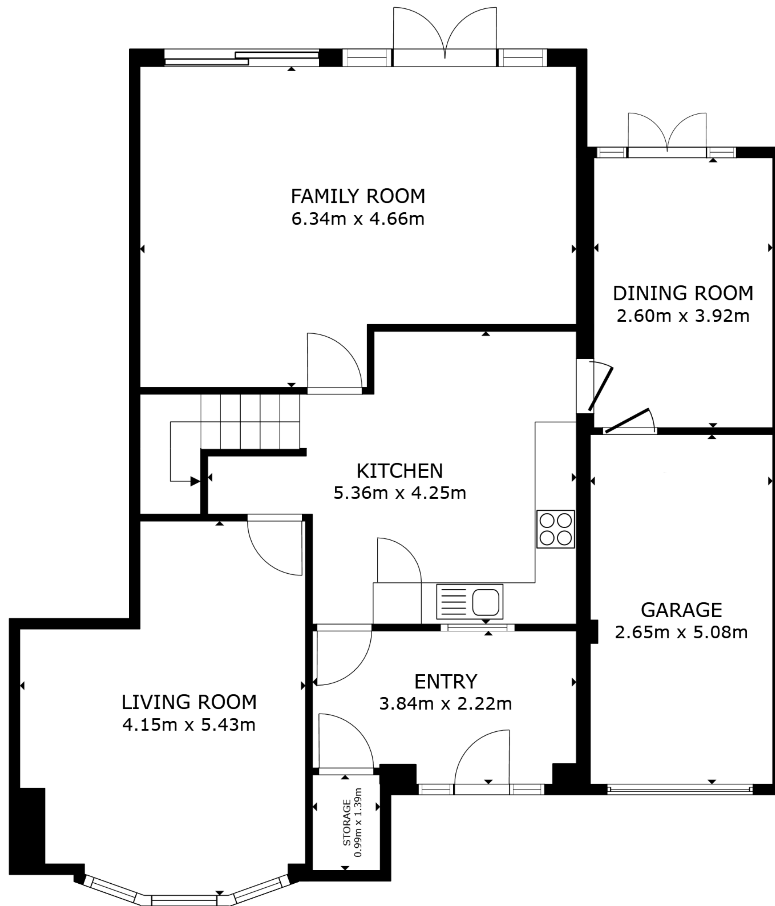
FLOOR 1
