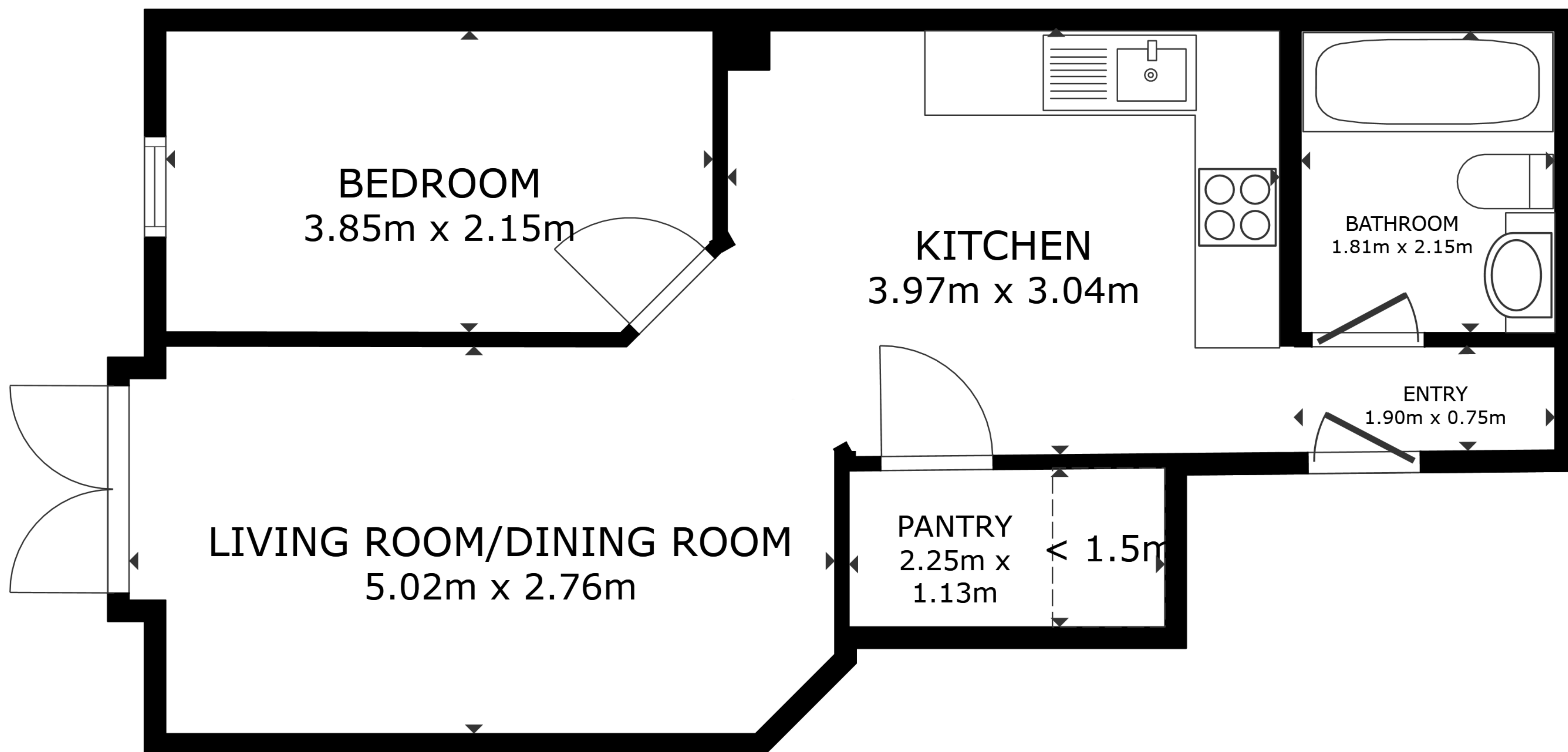
FLOOR PLAN
