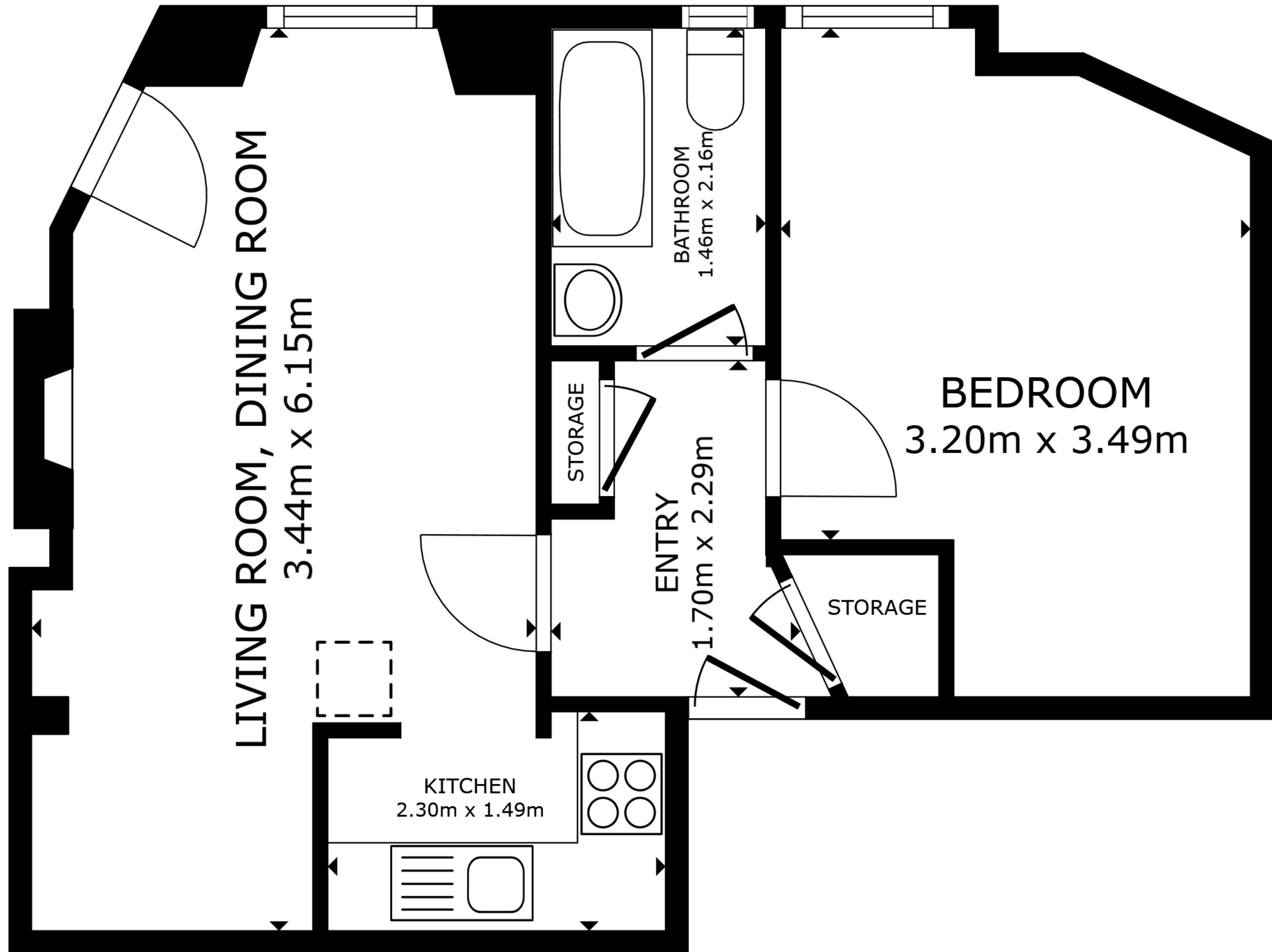
FLOOR PLAN
