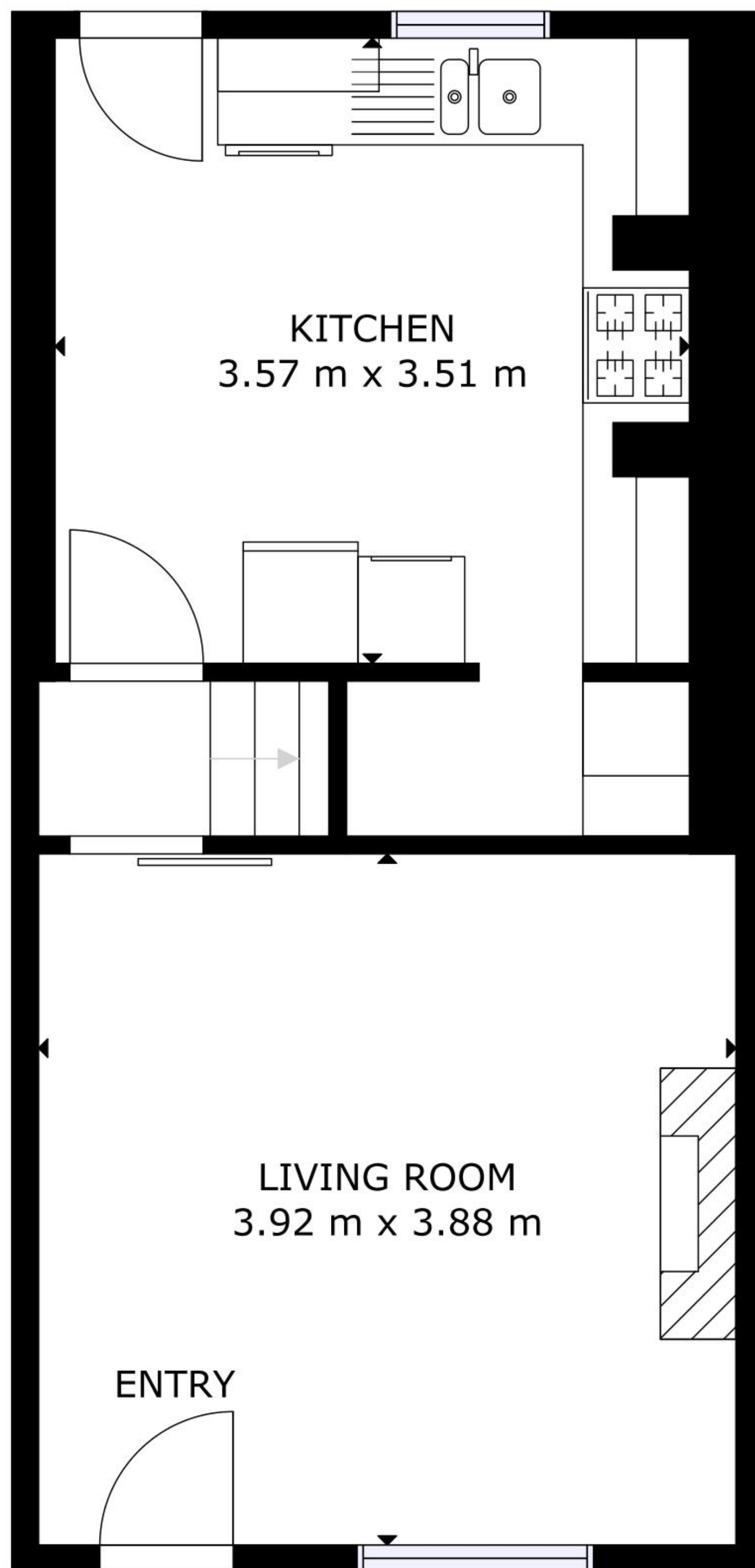
FLOOR 1
