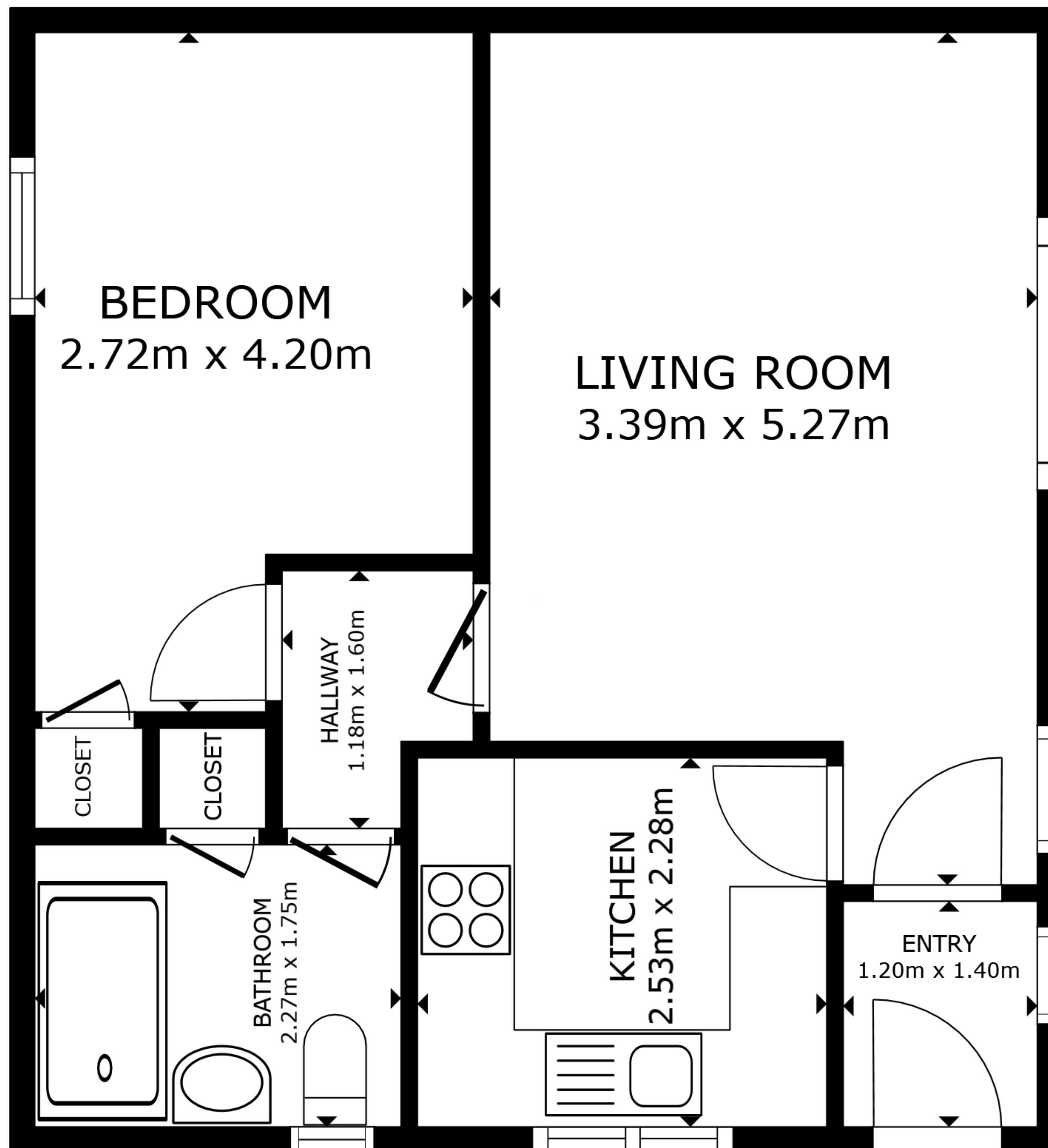
FLOOR PLAN
