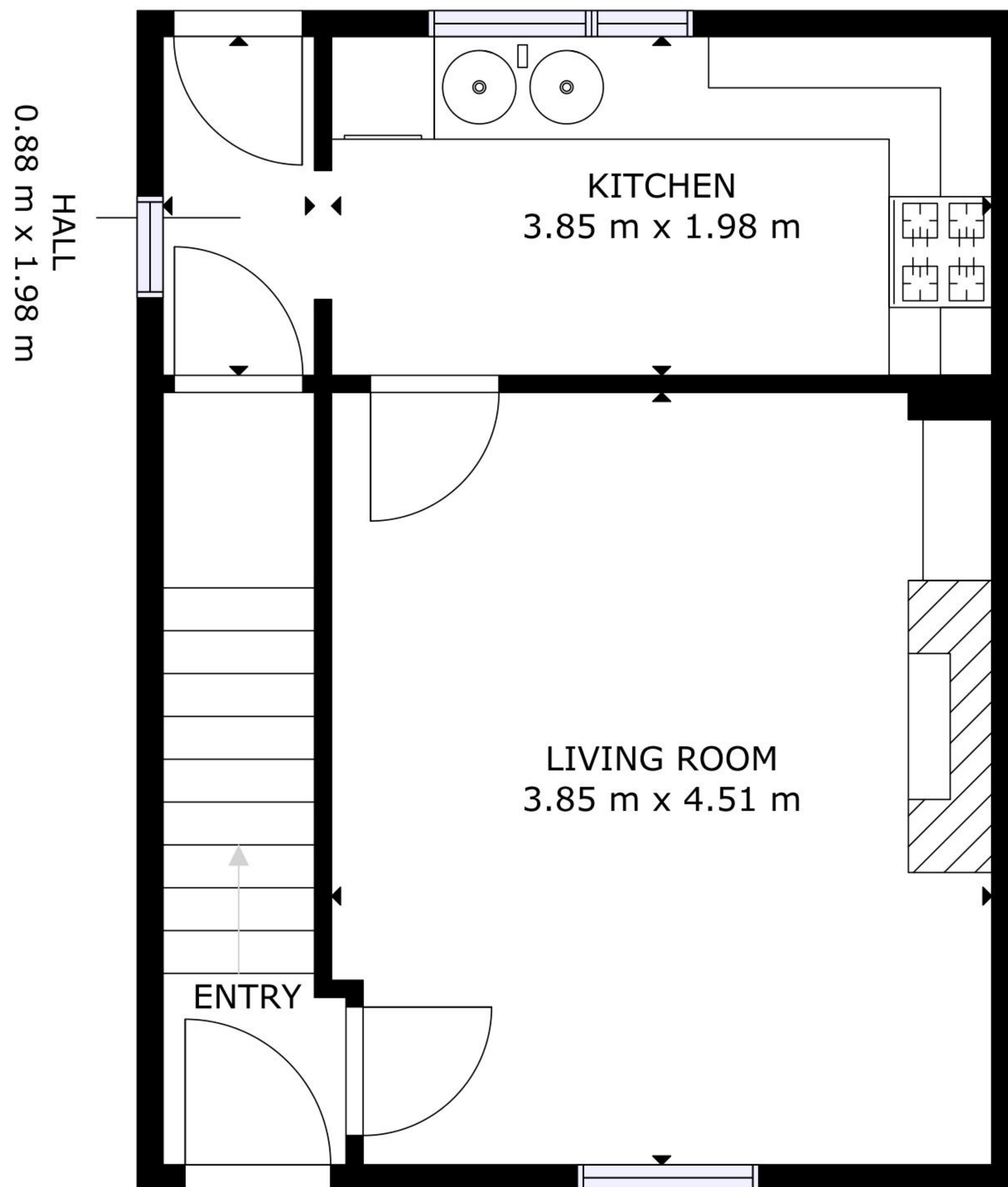
FLOOR 1
