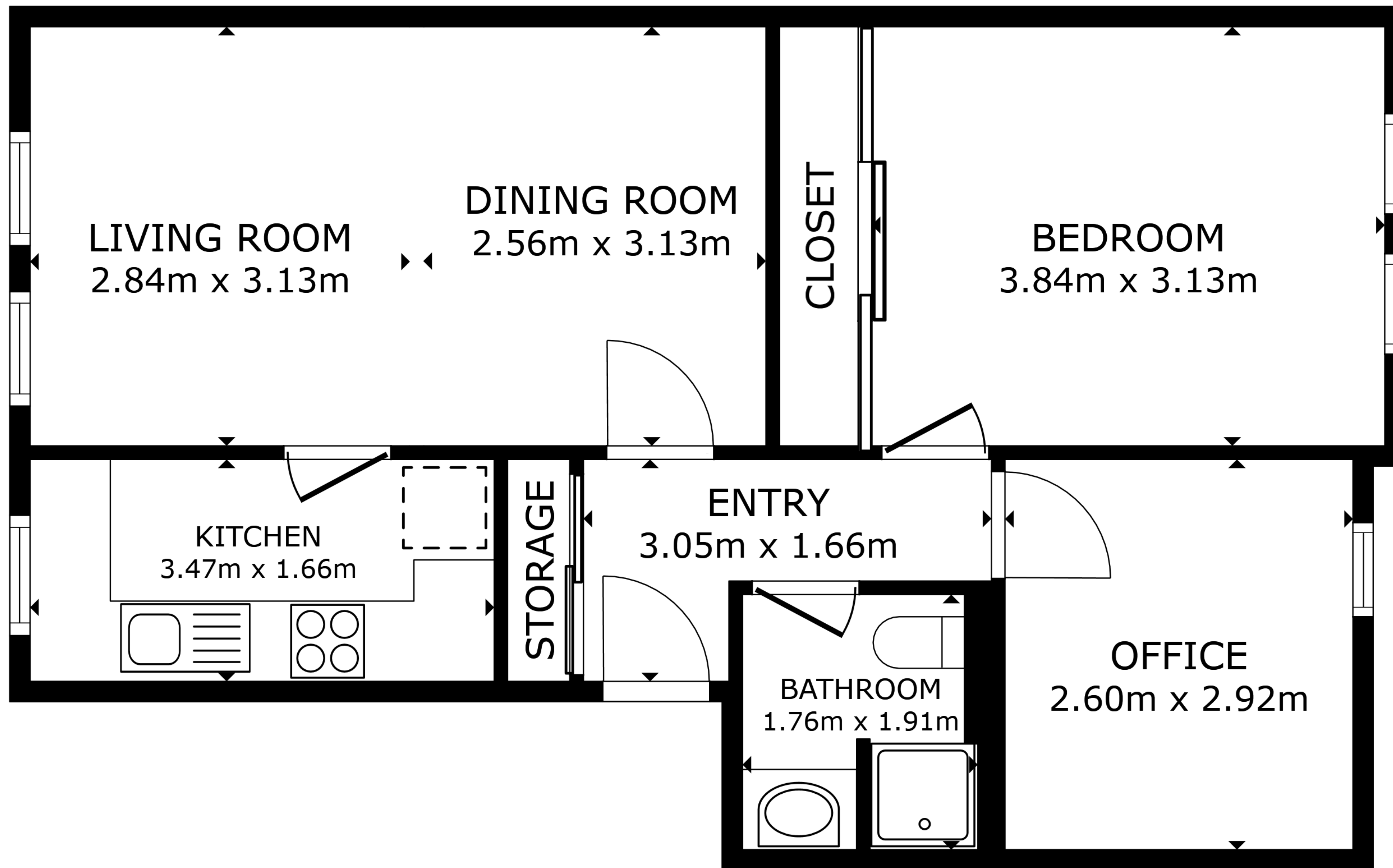
FLOOR PLAN
