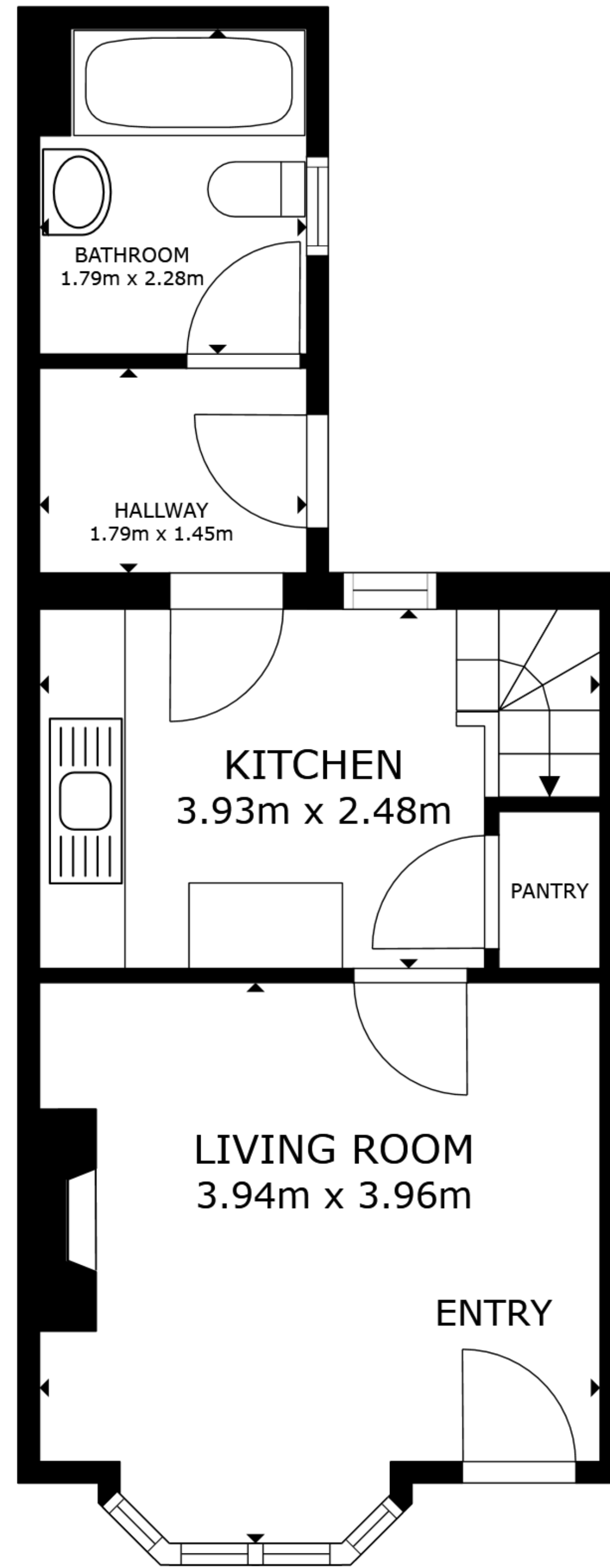
FLOOR 1
