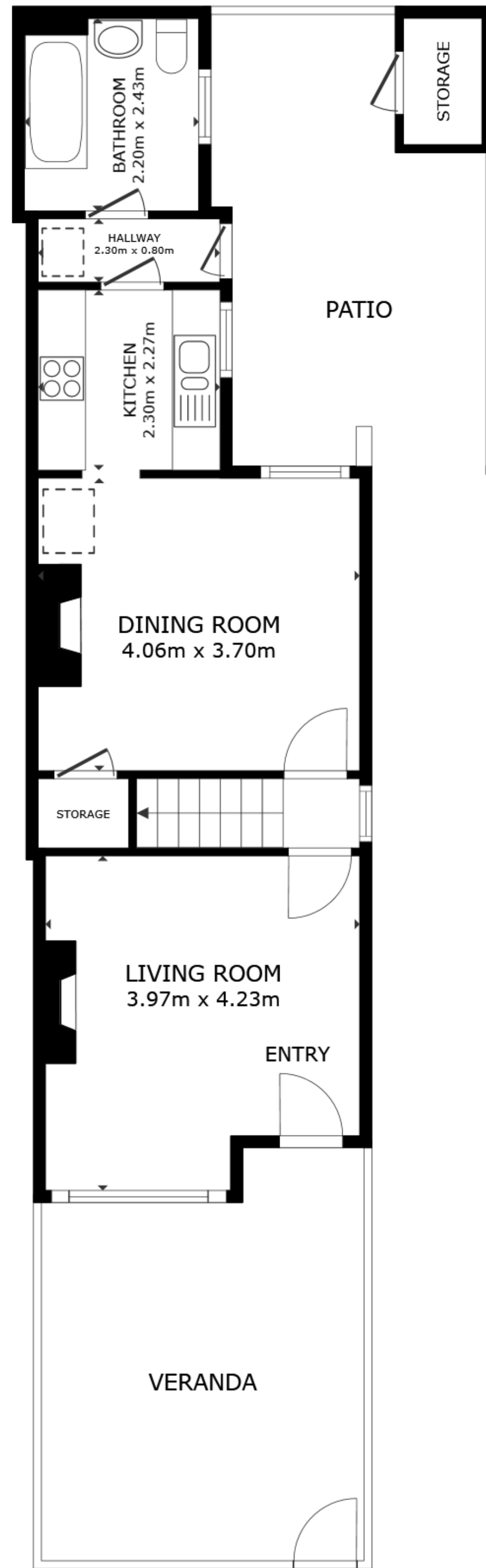
FLOOR 1
