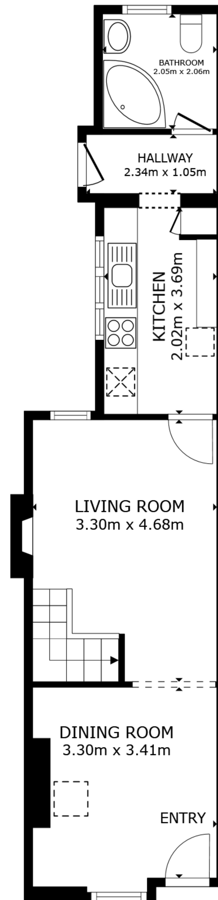
FLOOR 1
