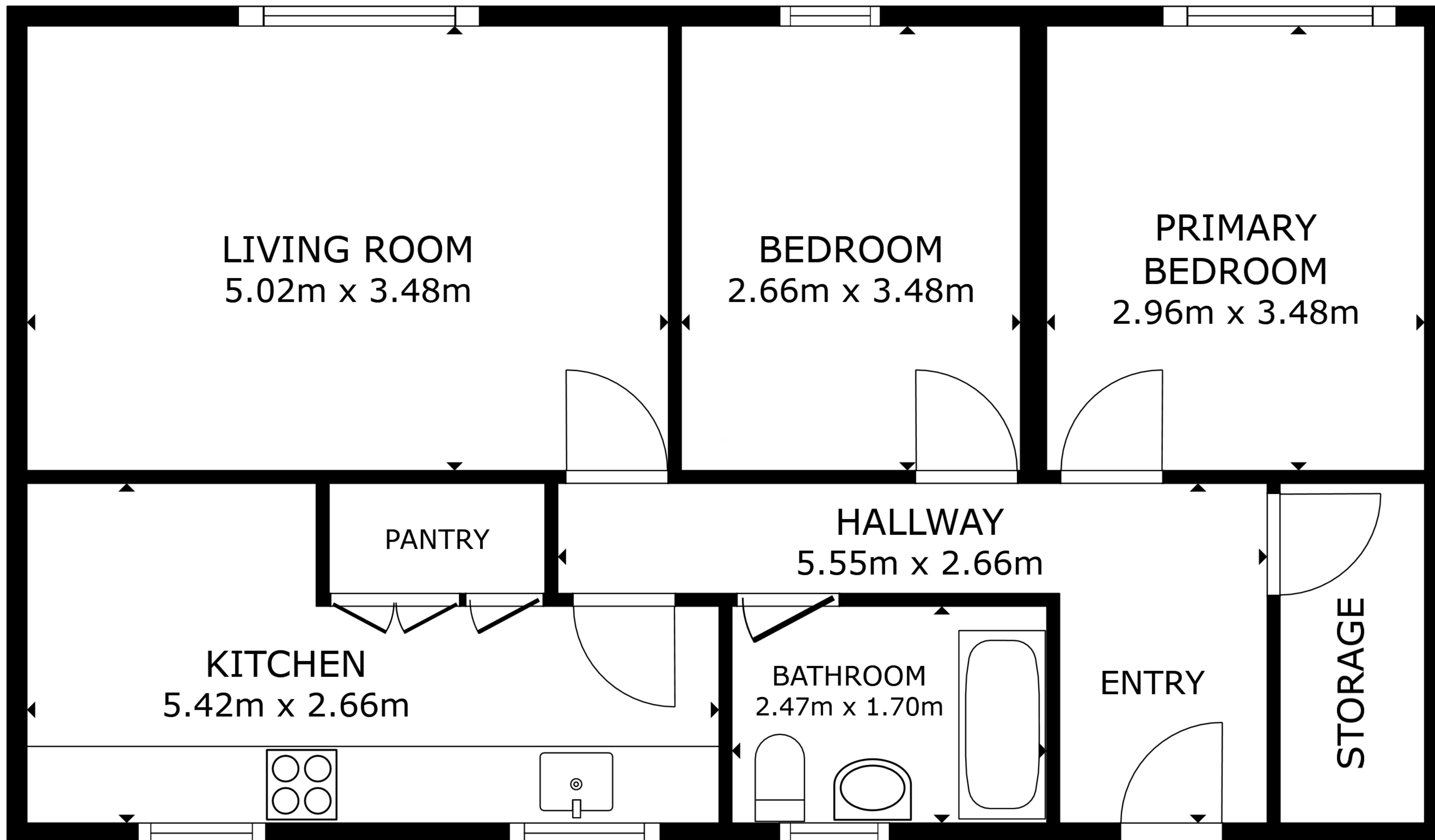
FLOOR PLAN
