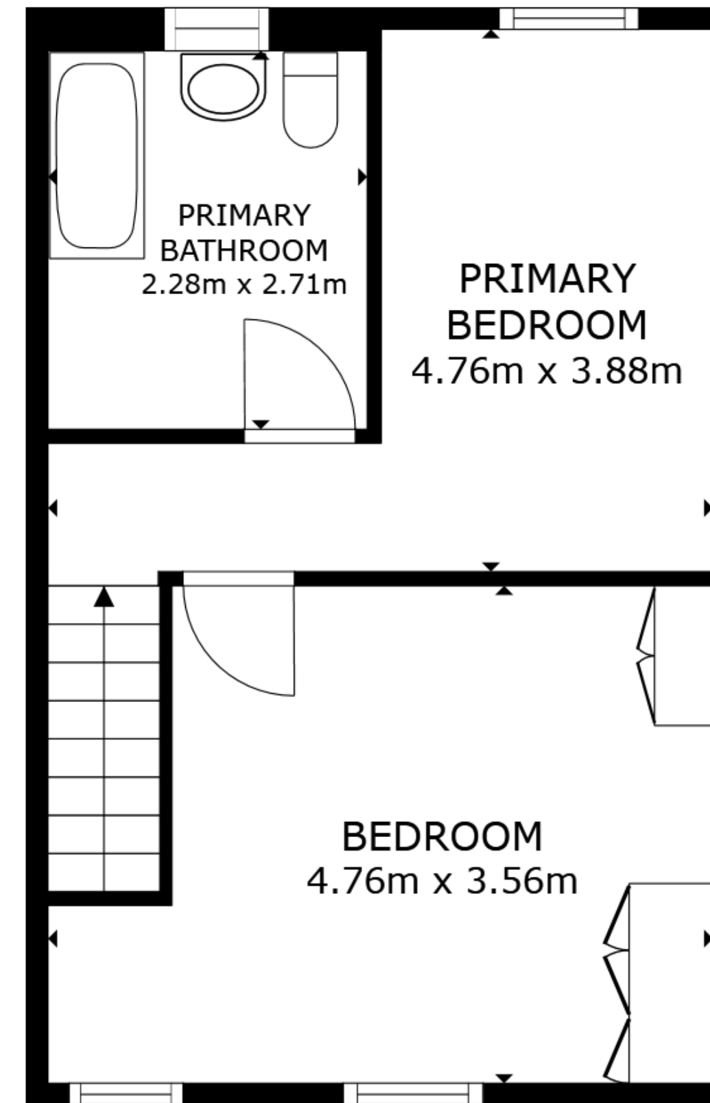
FLOOR 2
