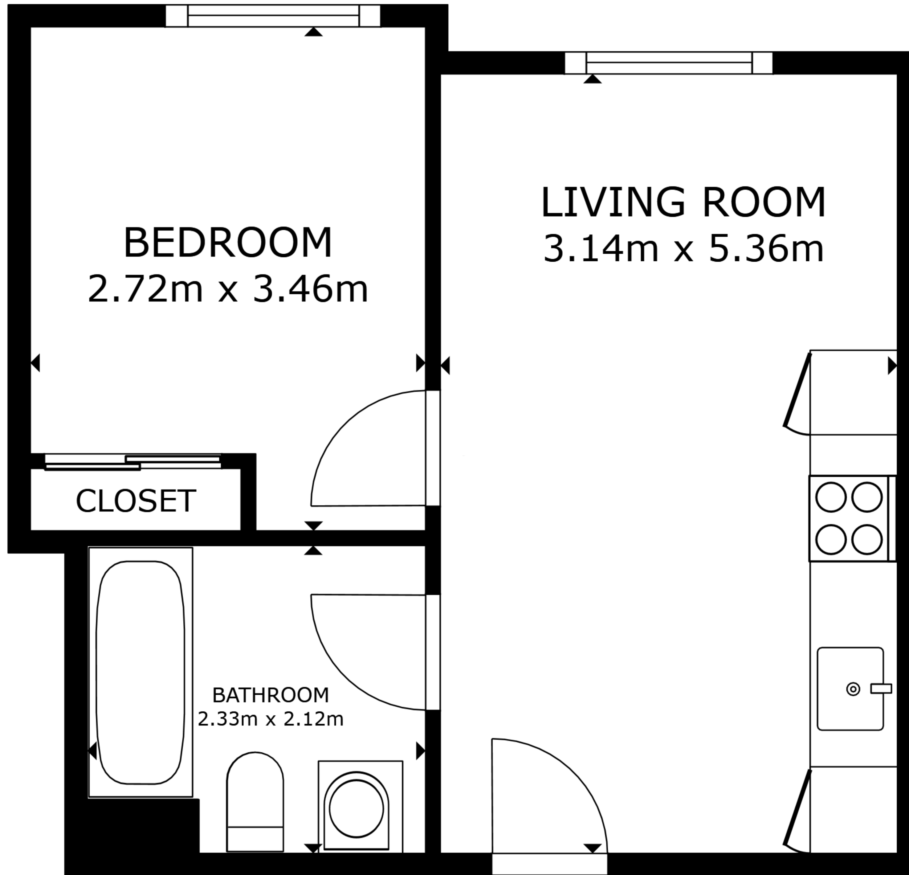
FLOOR PLAN
