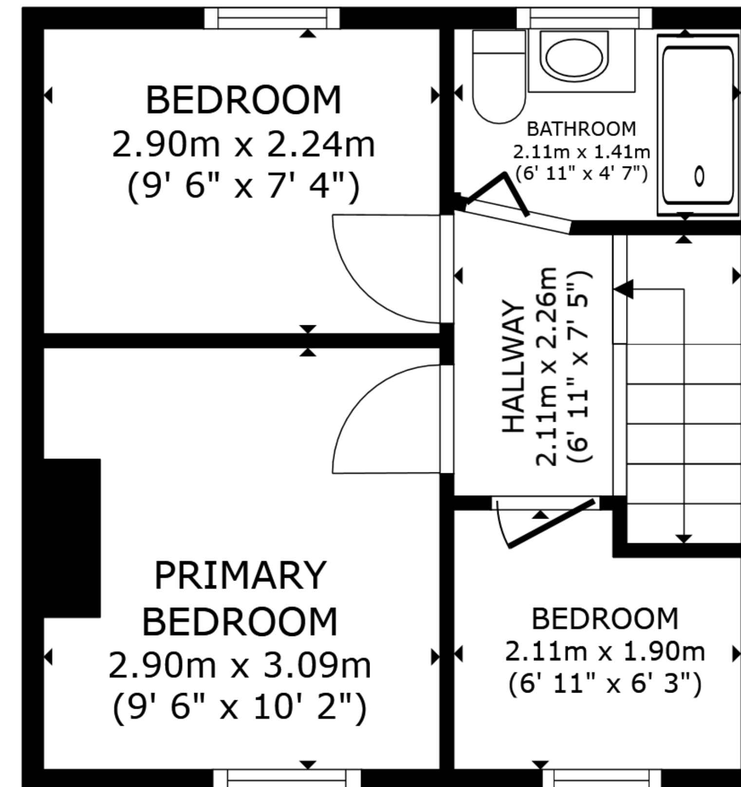
FLOOR 2
