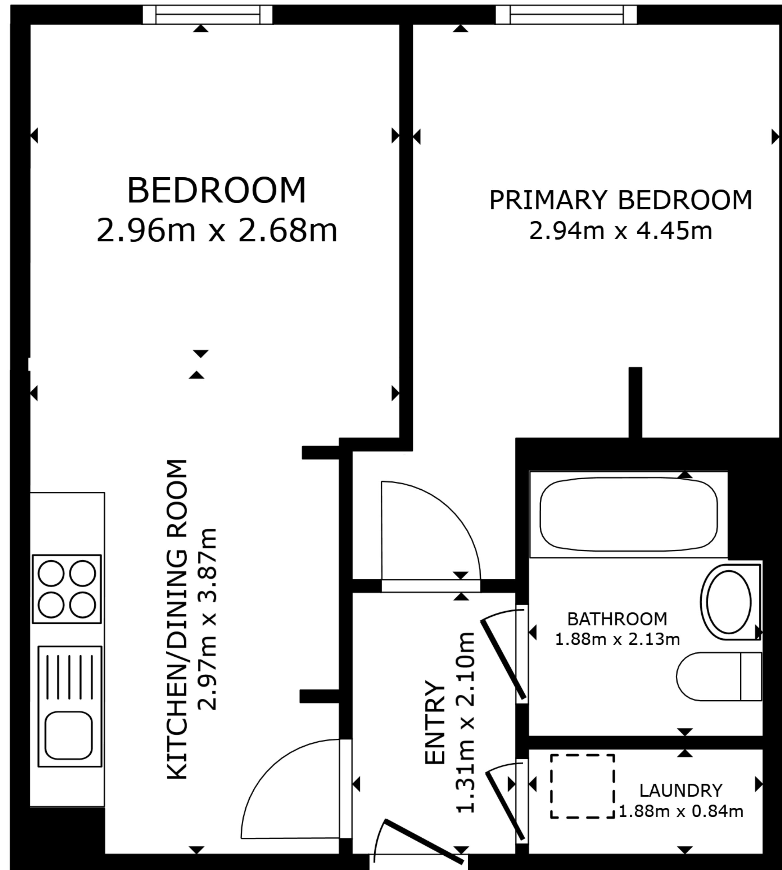
FLOOR PLAN
