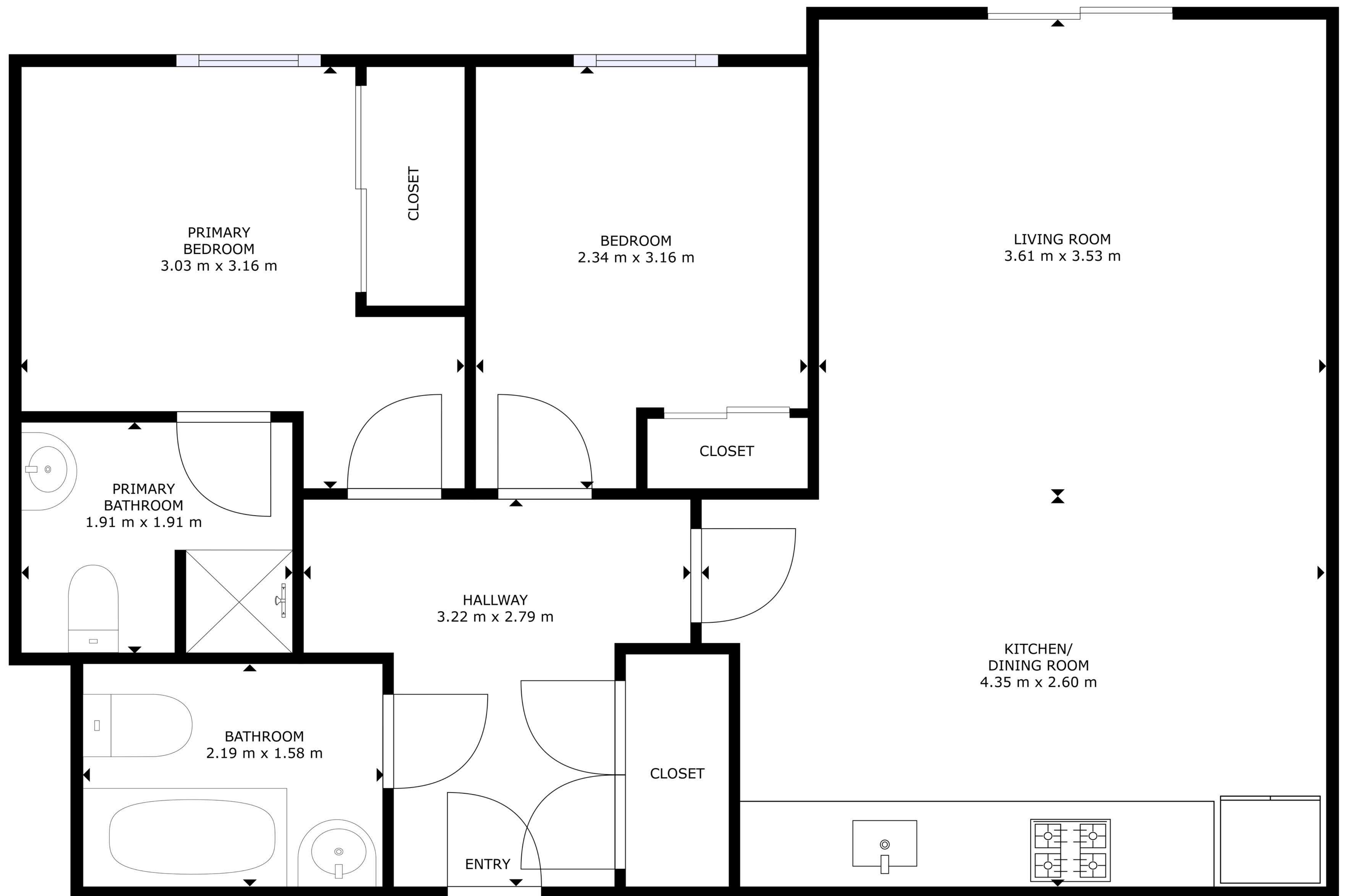
FLOOR PLAN
