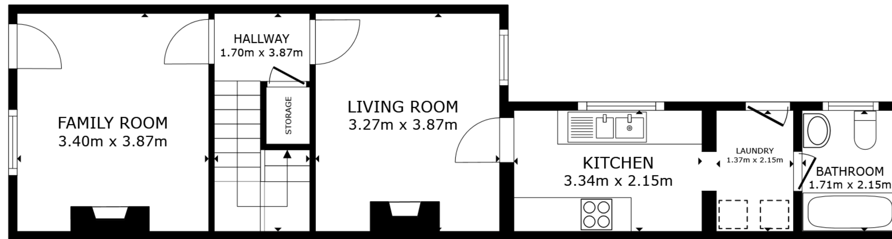
FLOOR 1
