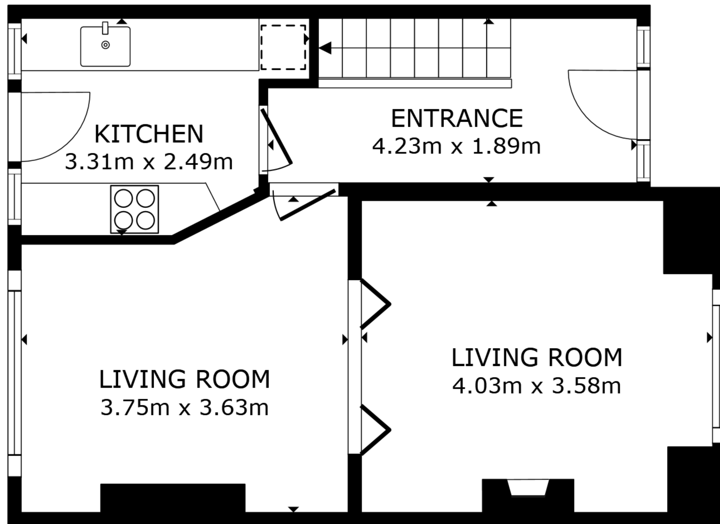
FLOOR 1
