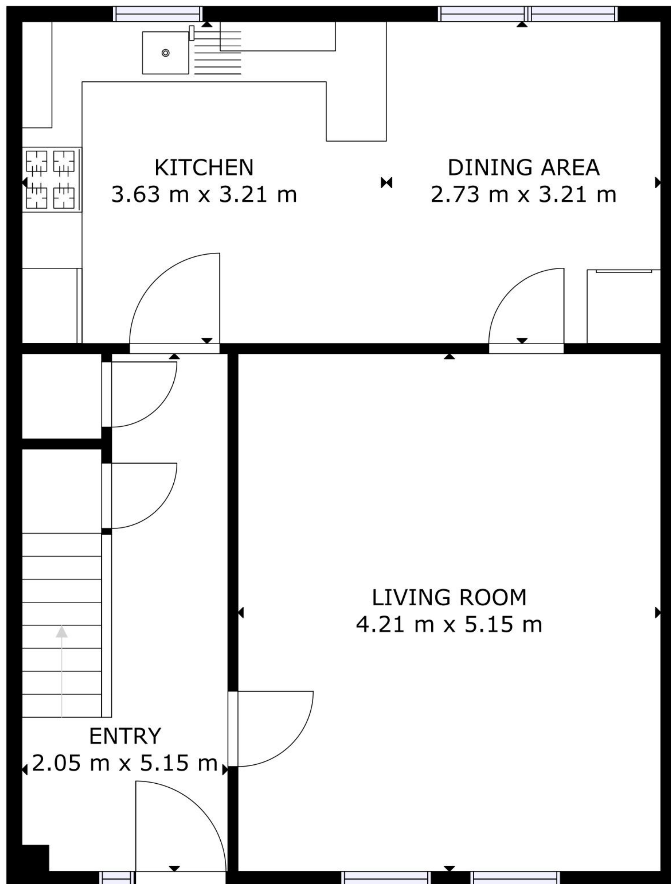
FLOOR 1
