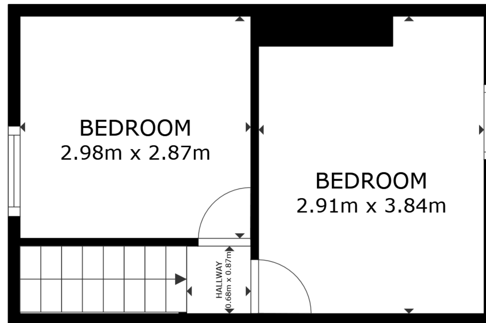
FLOOR 2
