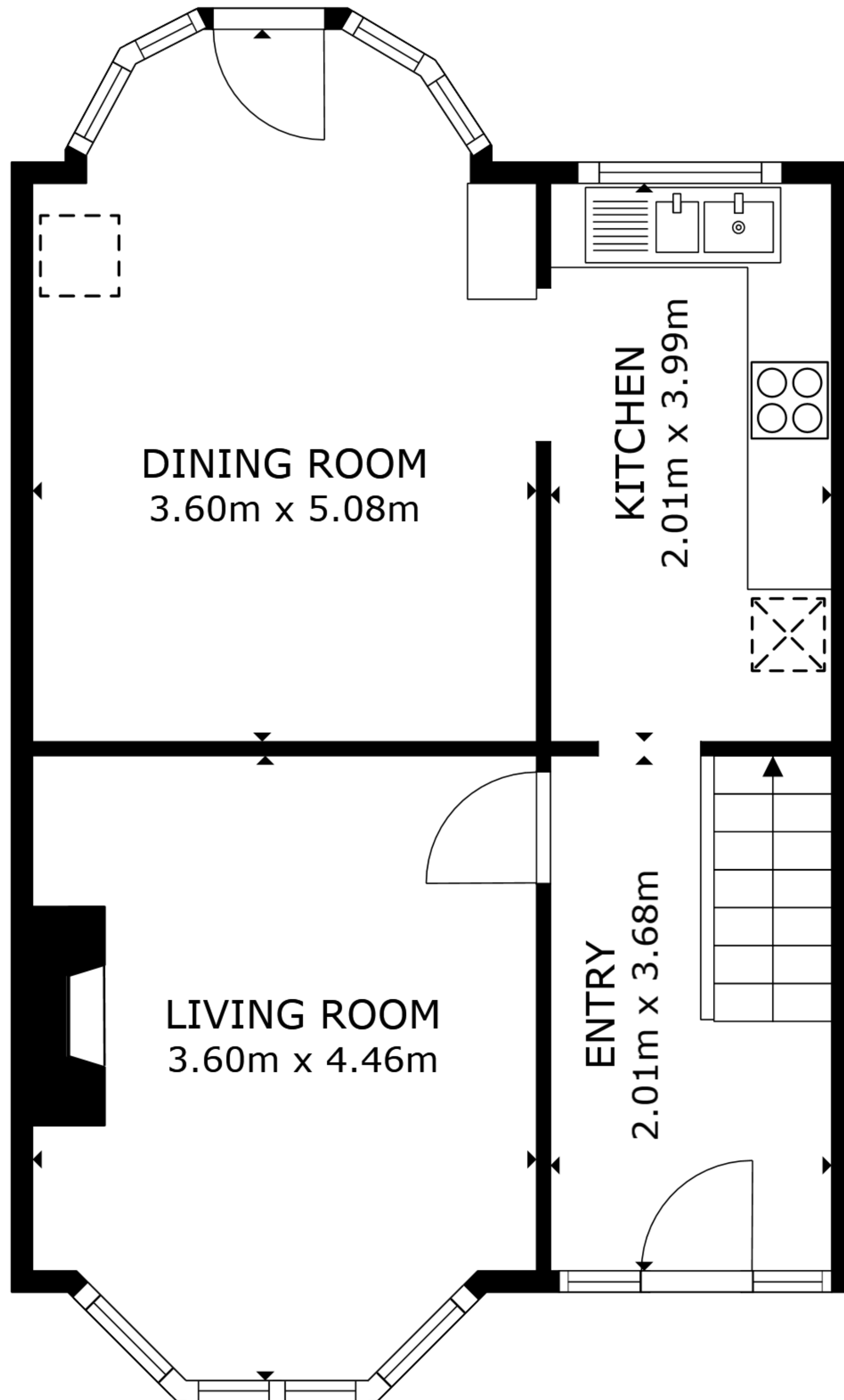
FLOOR 1
