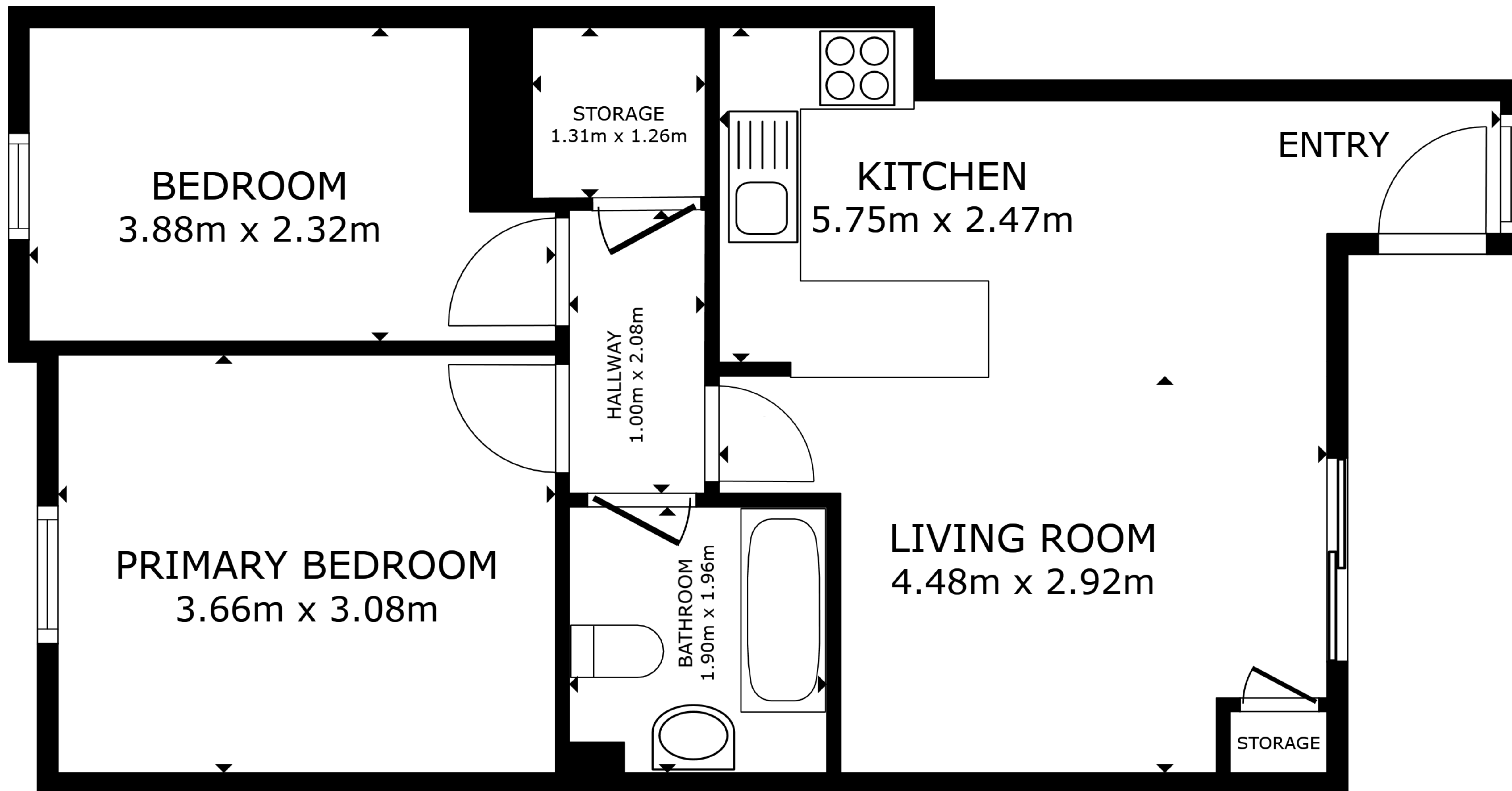
FLOOR PLAN
