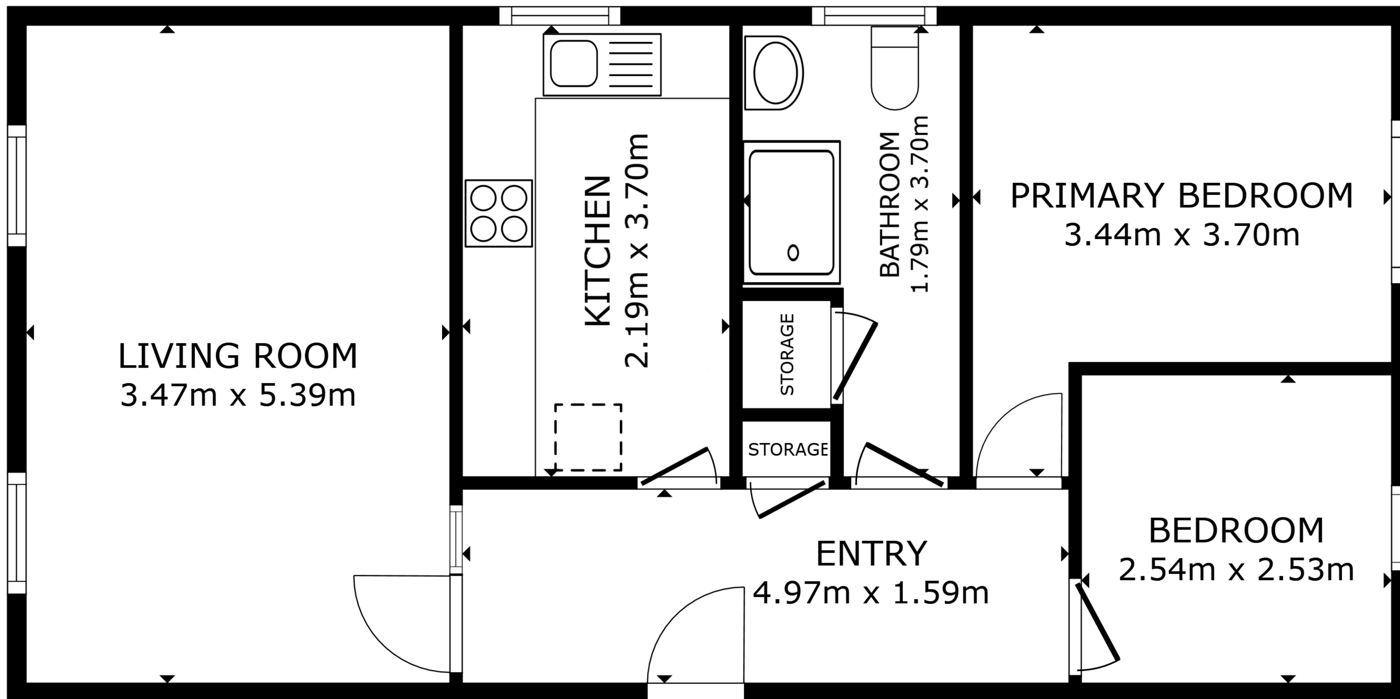
FLOOR PLAN
