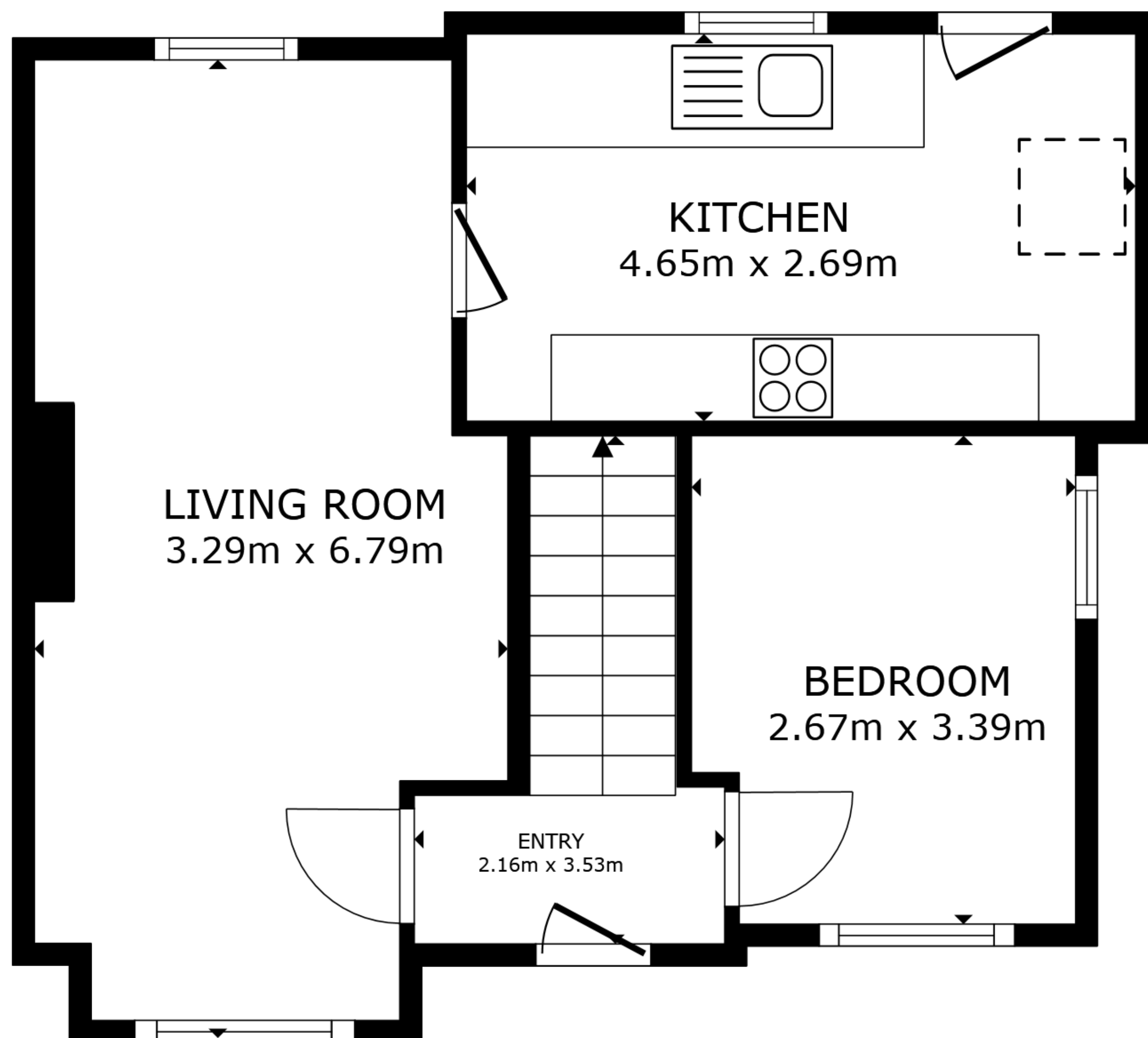
FLOOR 1
