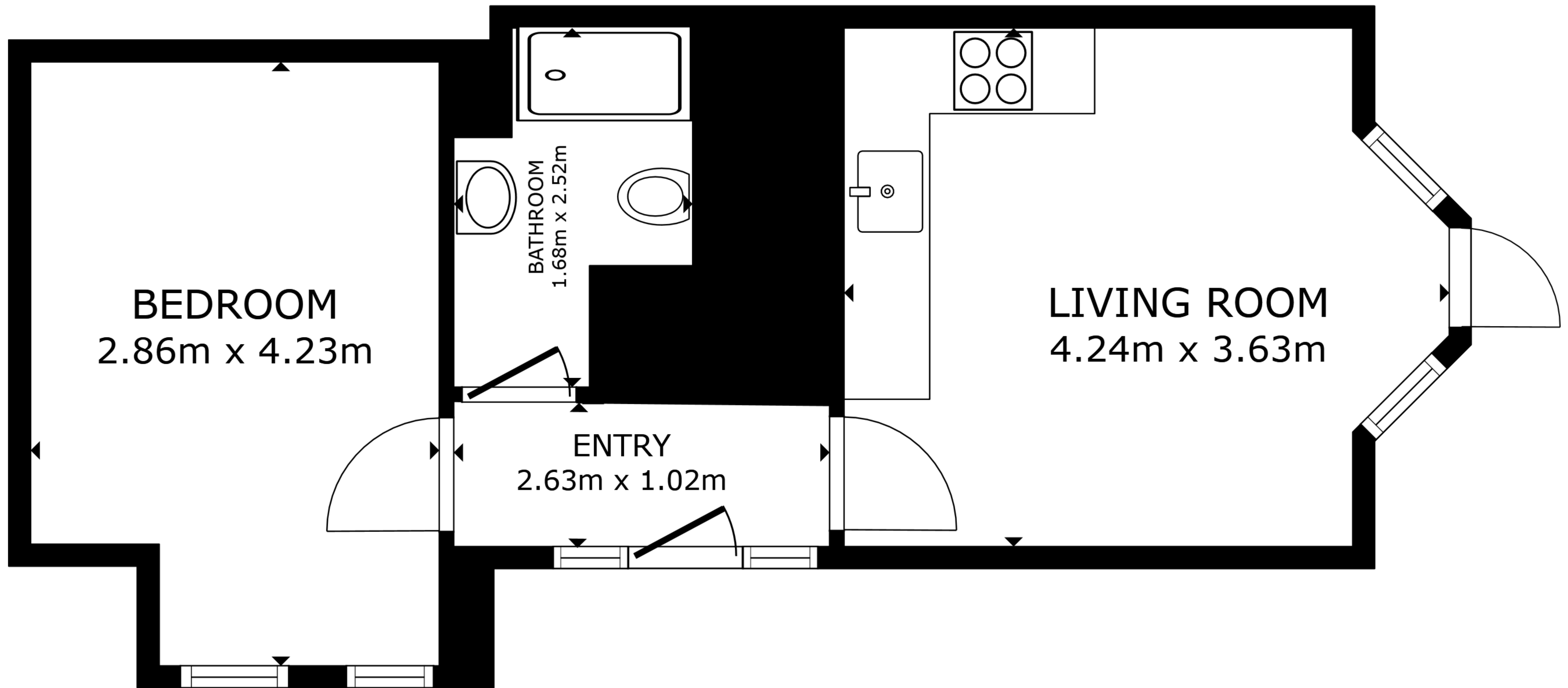
FLOOR PLAN
