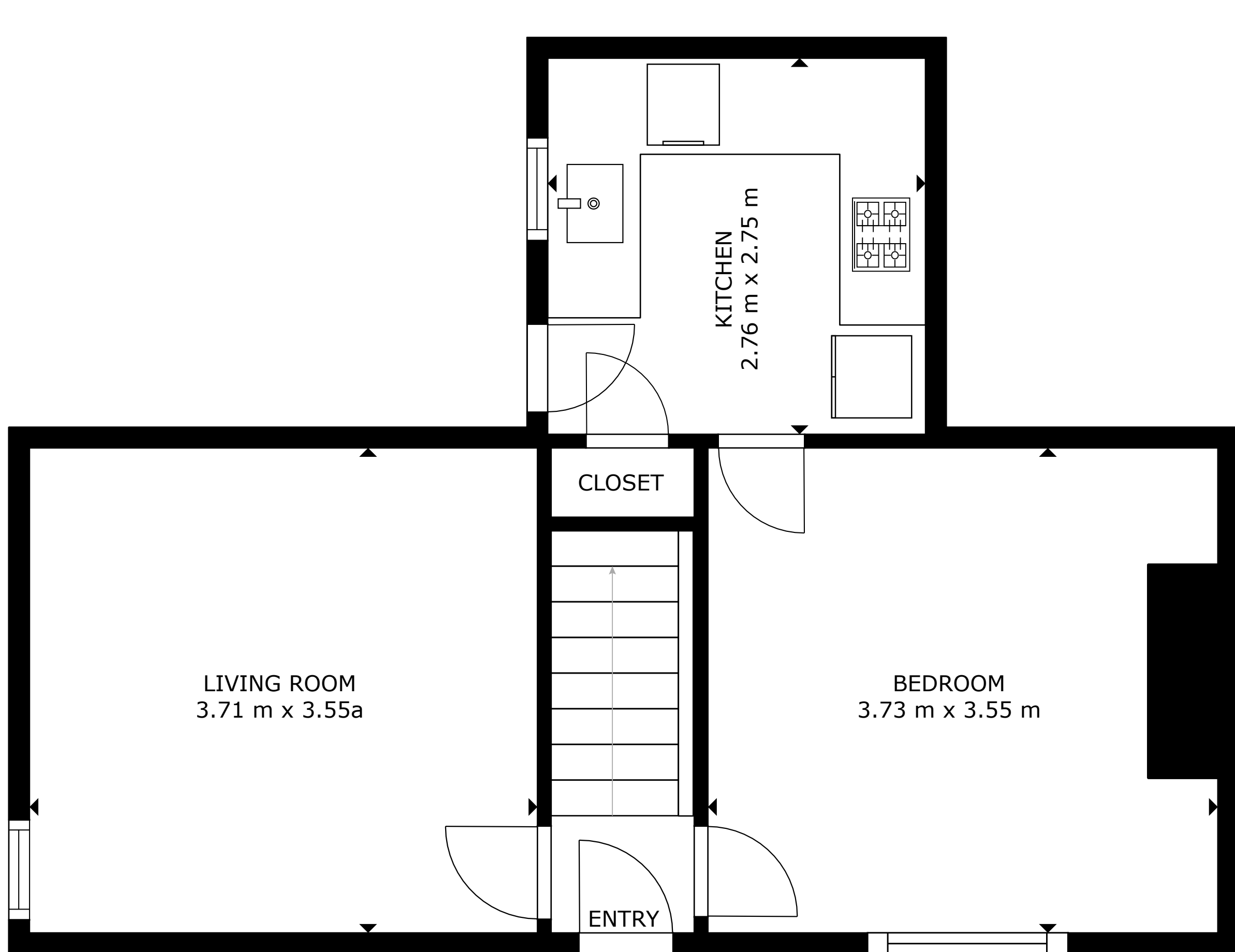
FLOOR 1
