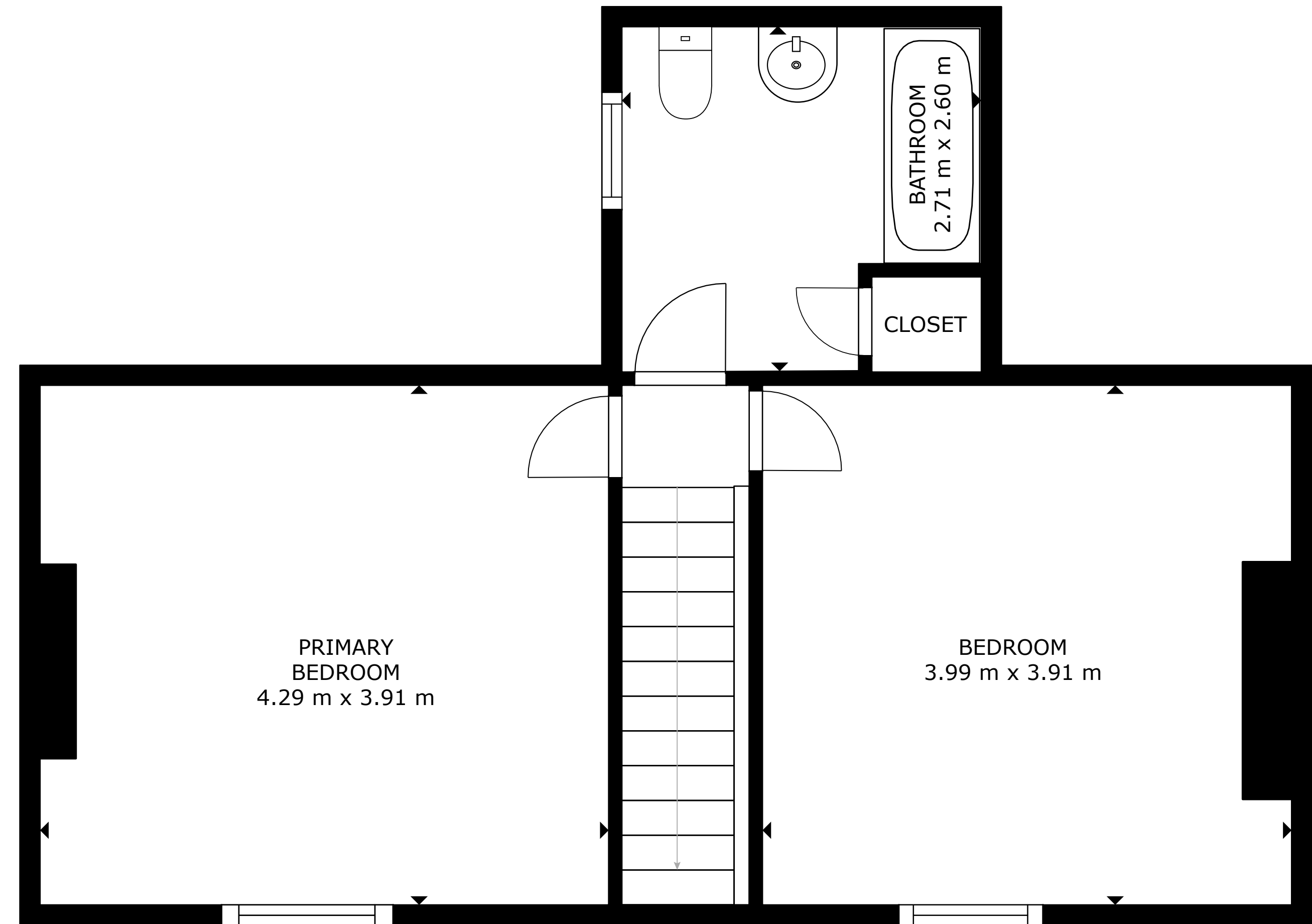
FLOOR 2
