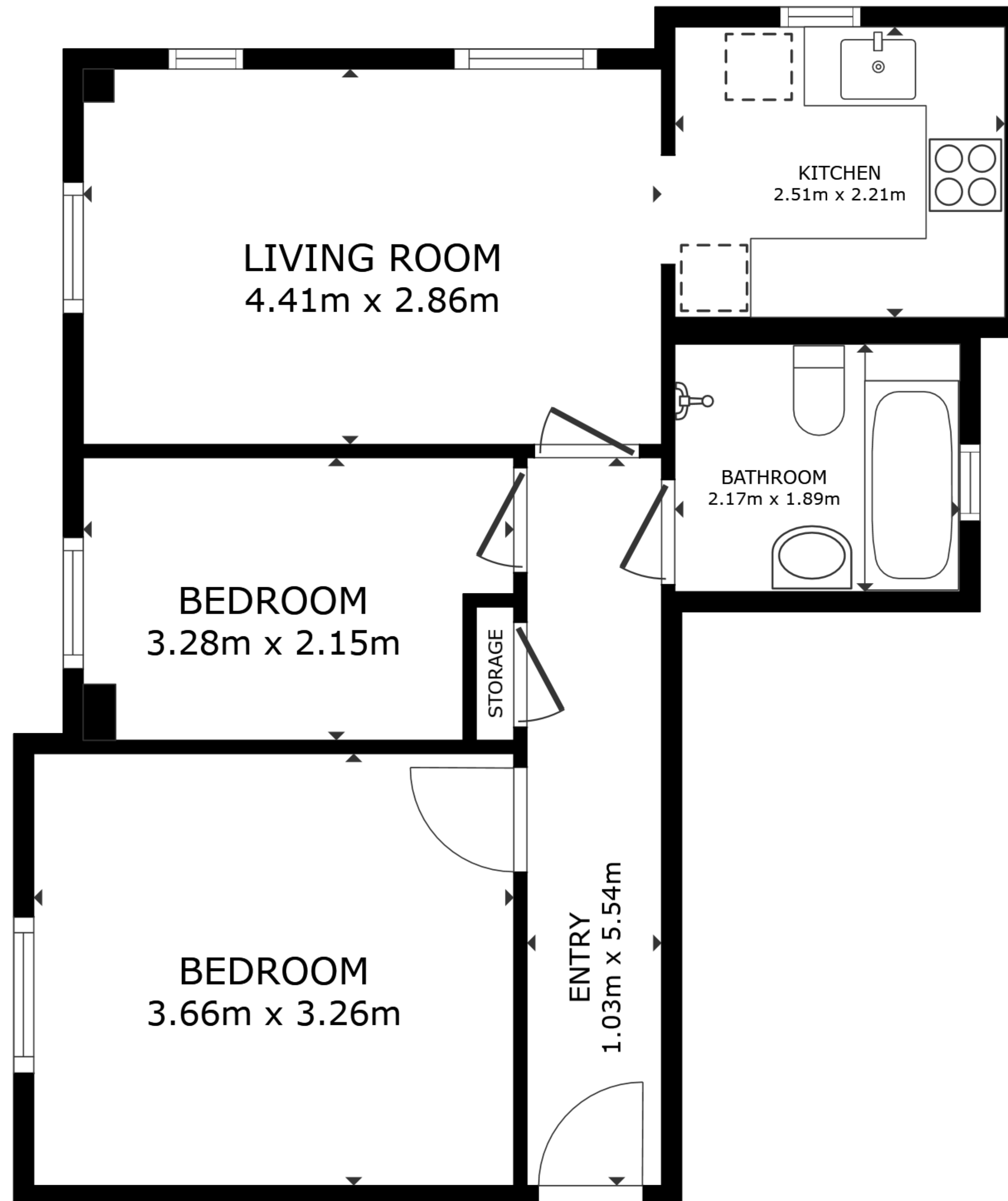
FLOOR PLAN
