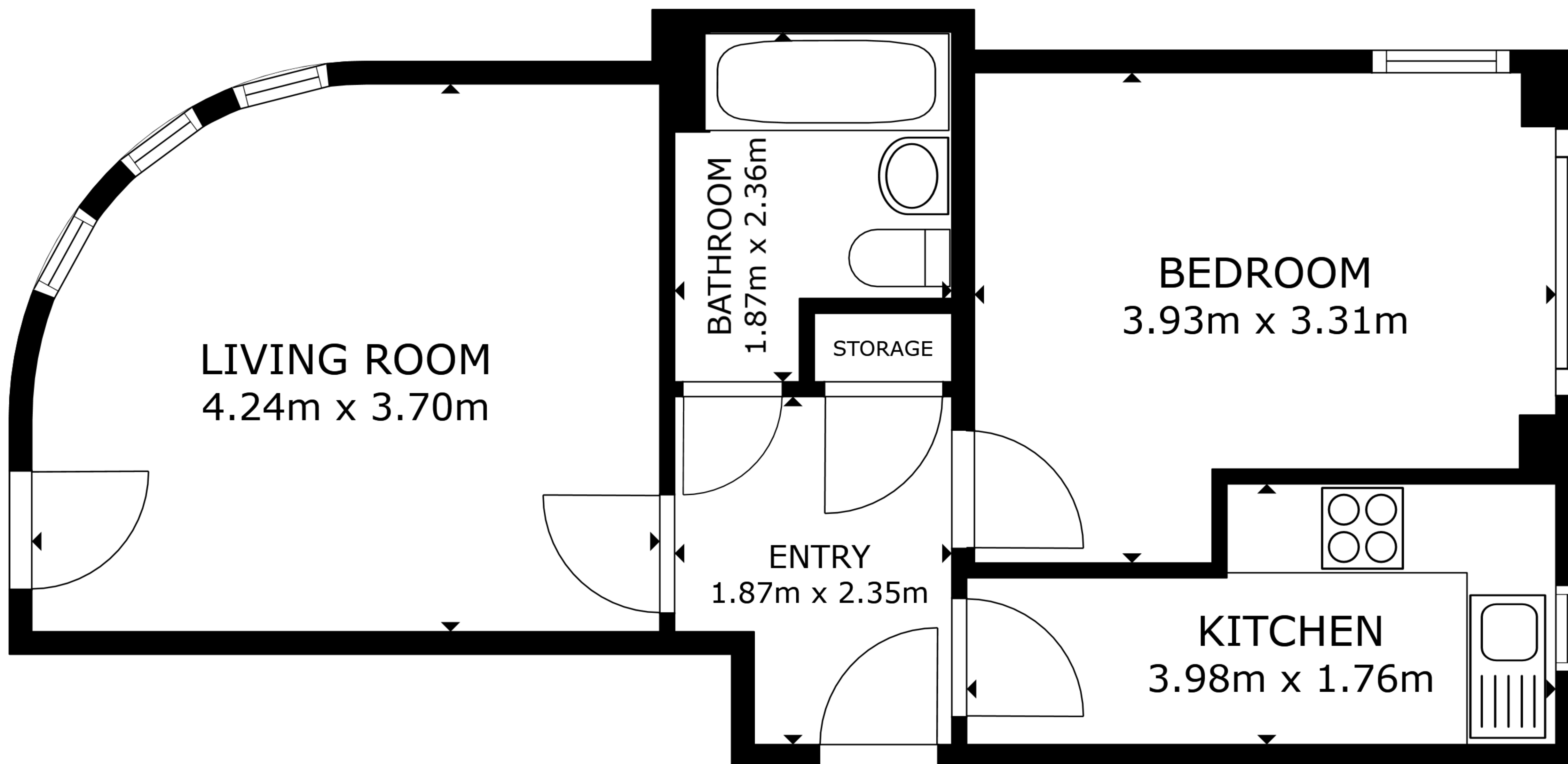
FLOOR PLAN
