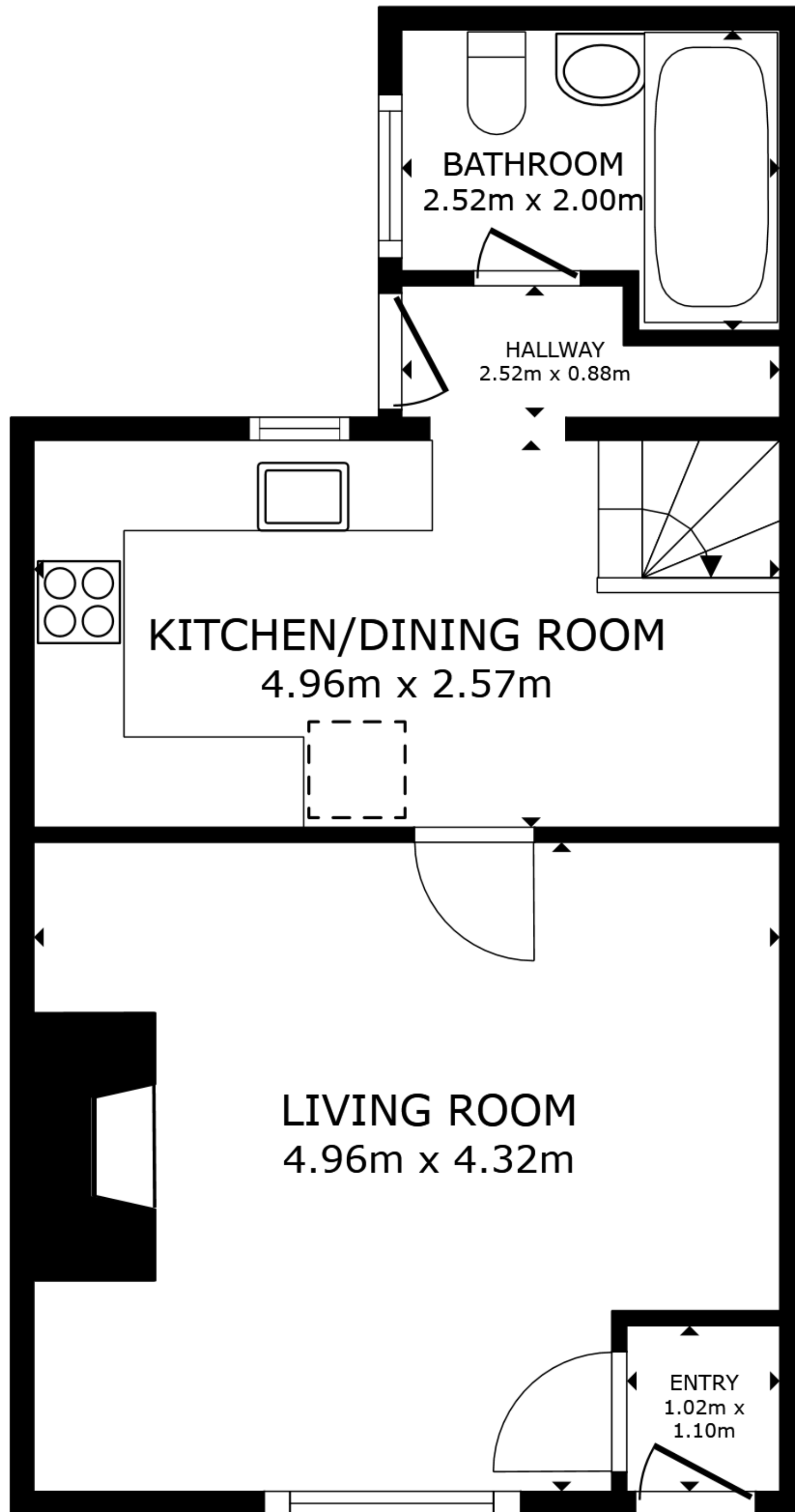
FLOOR 1
