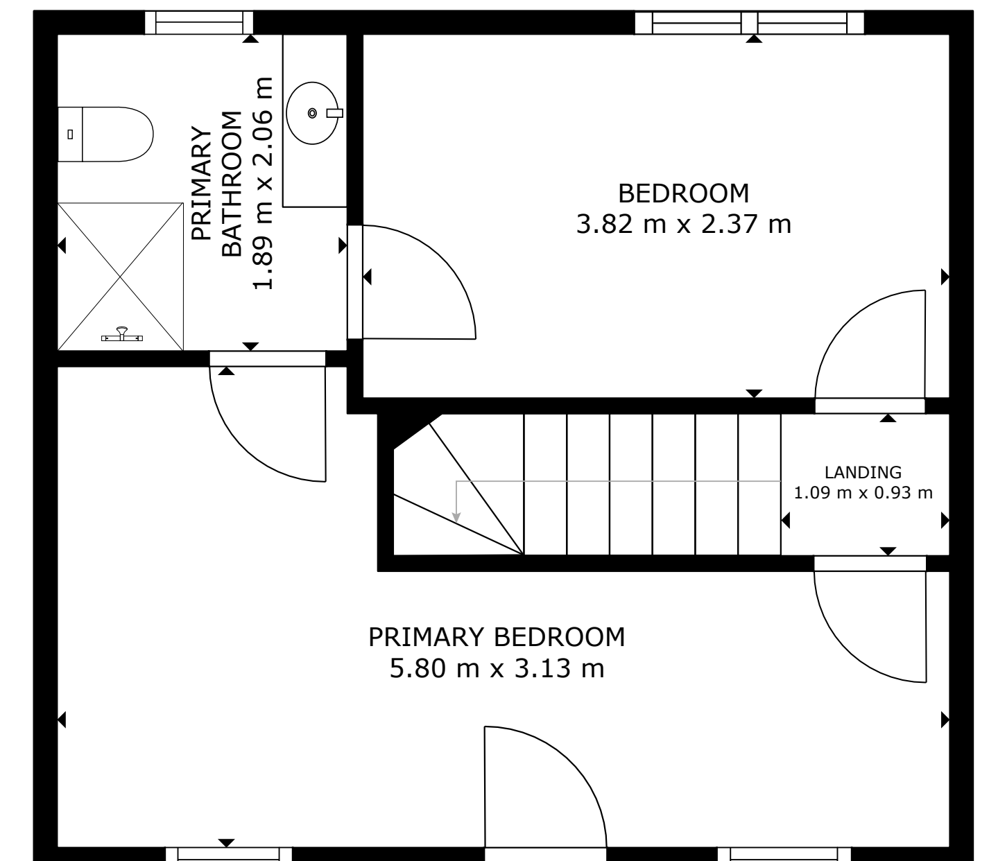
FLOOR 3
