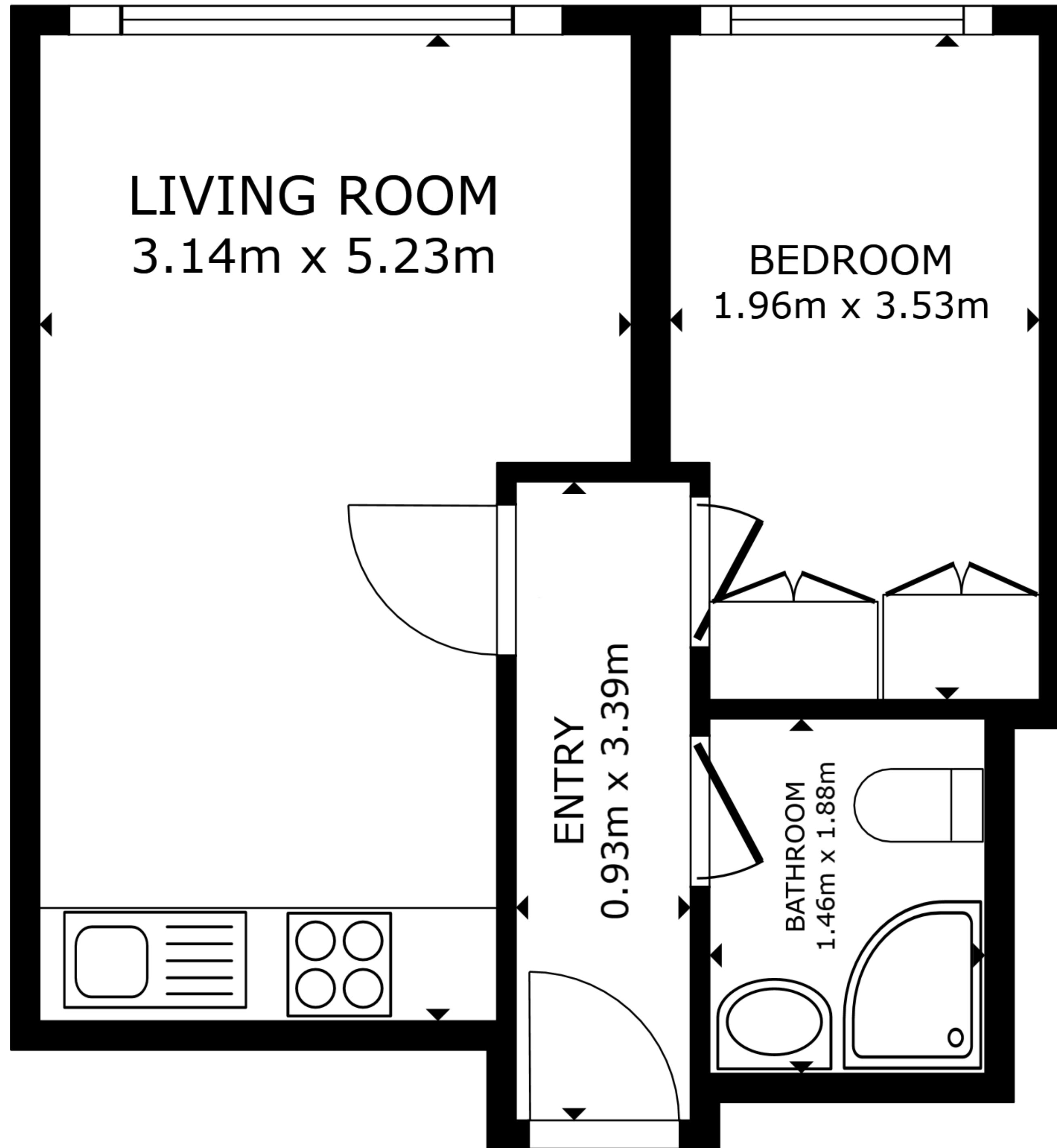
FLOOR PLAN
