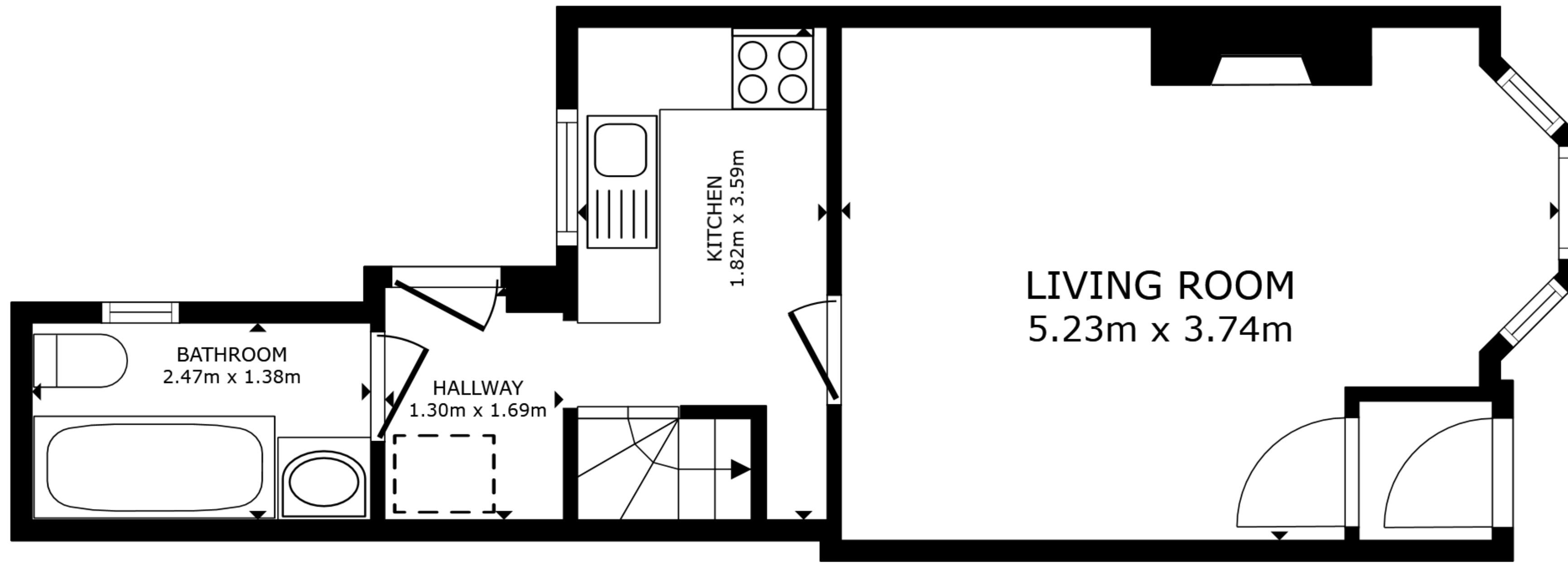
FLOOR 1
