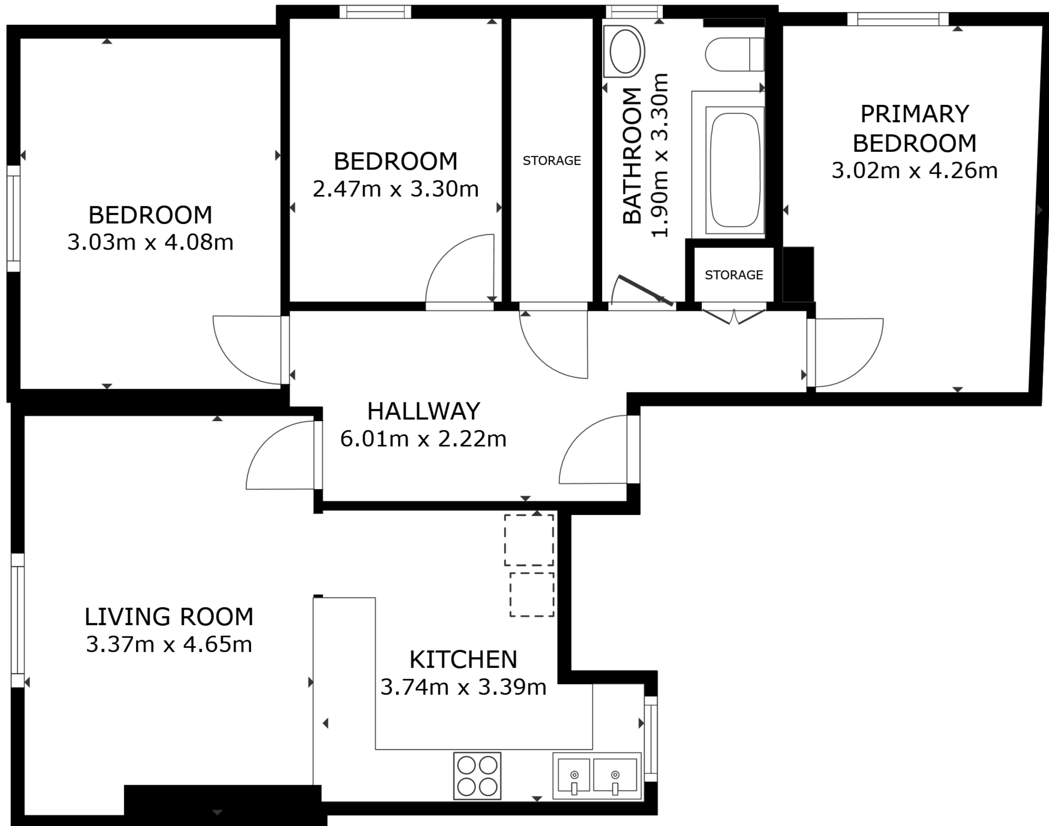
FLOOR PLAN
