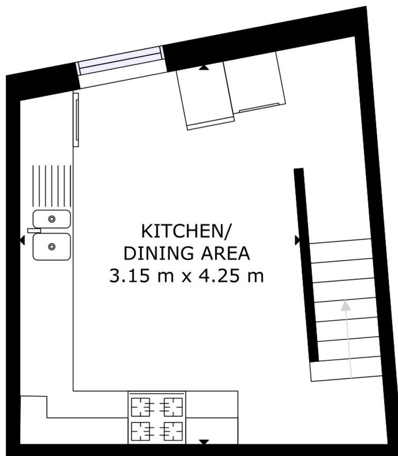
FLOOR 1
