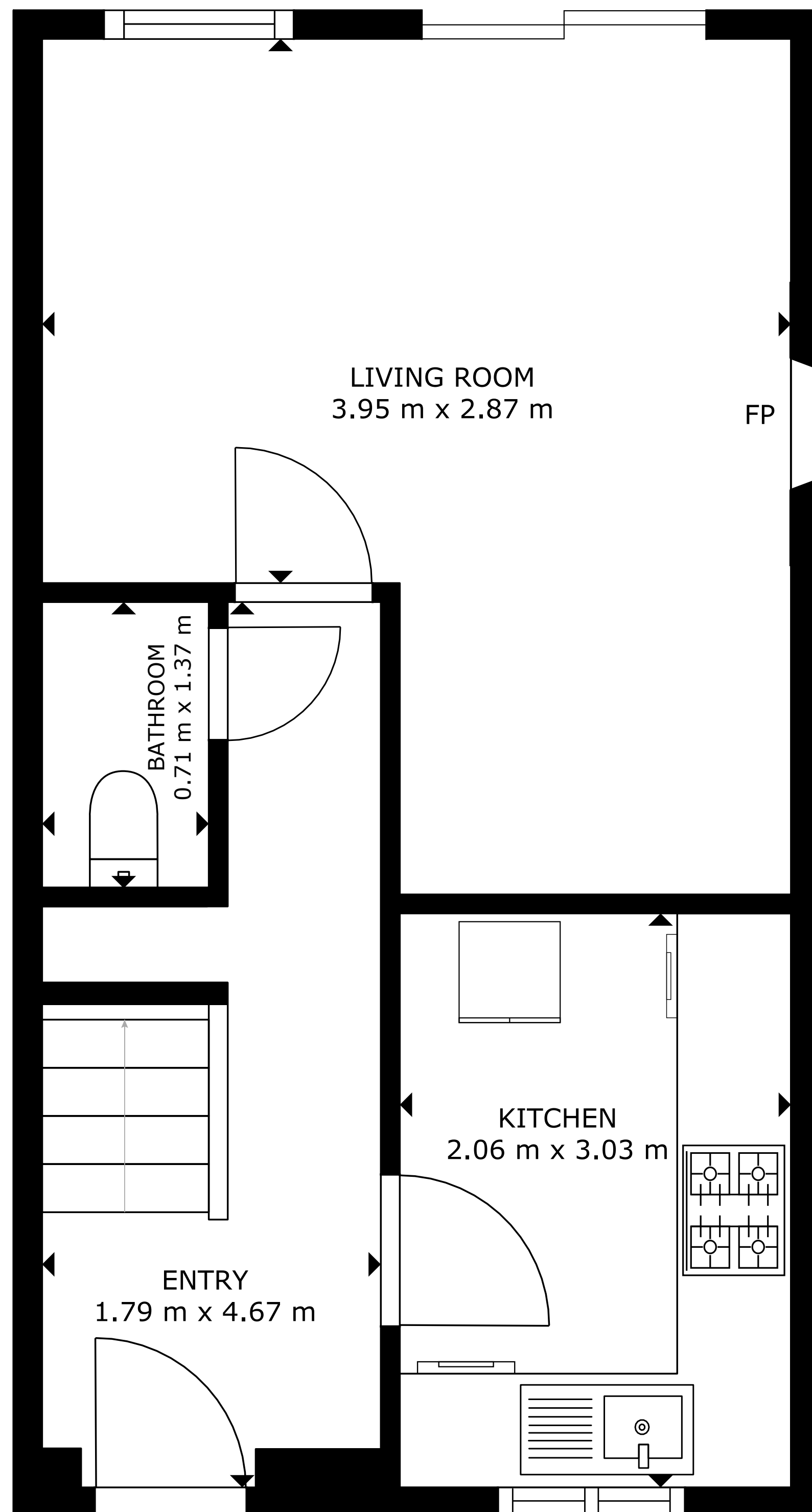
FLOOR 1
