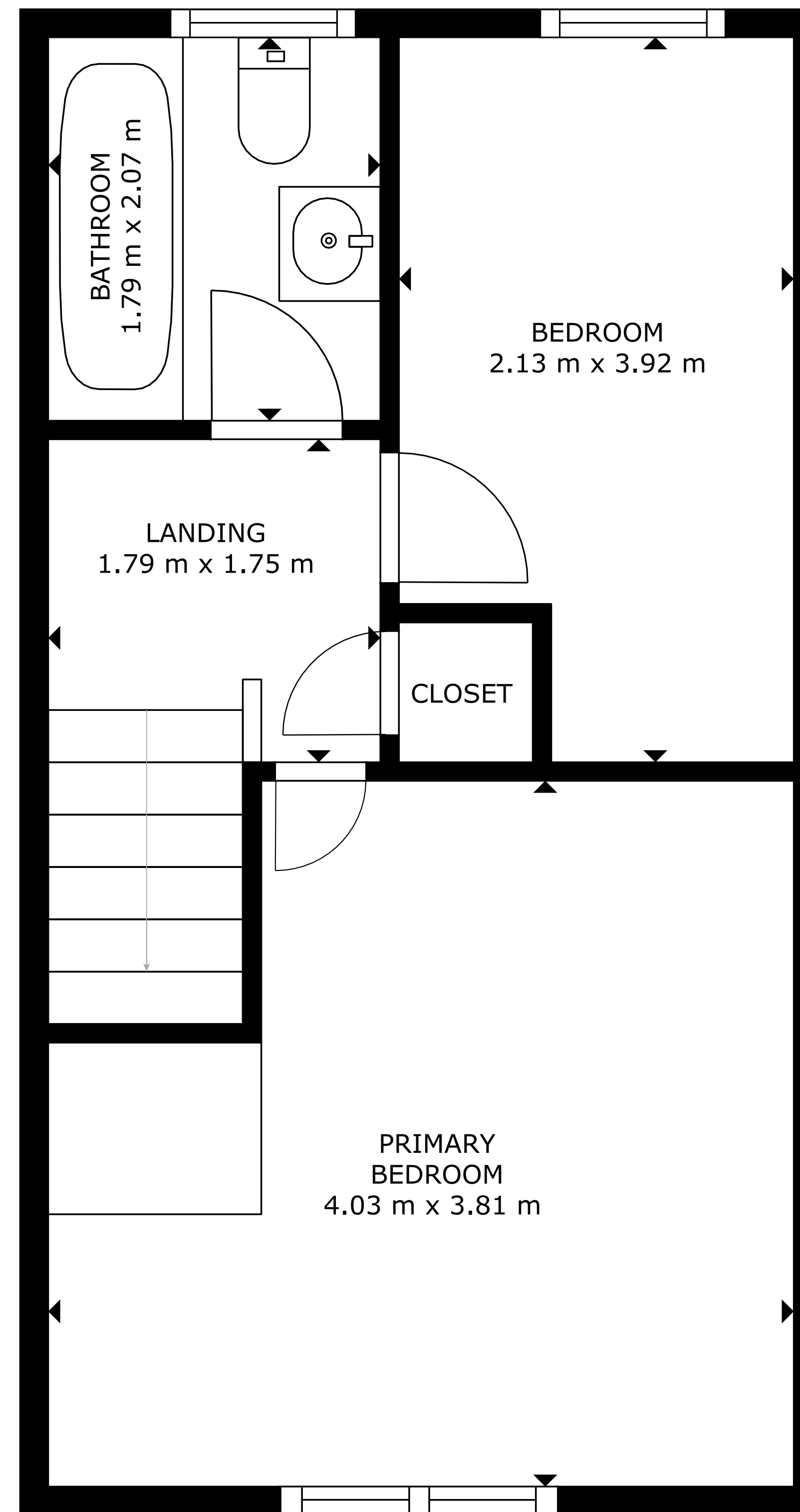
FLOOR 2
