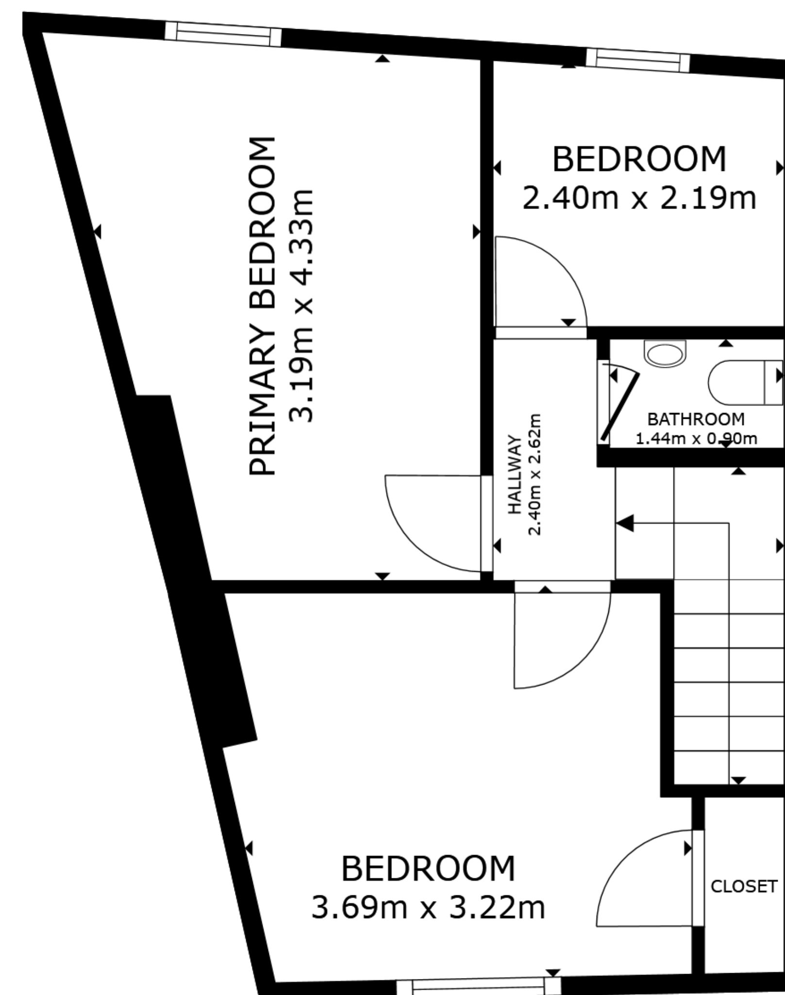
FLOOR 2
