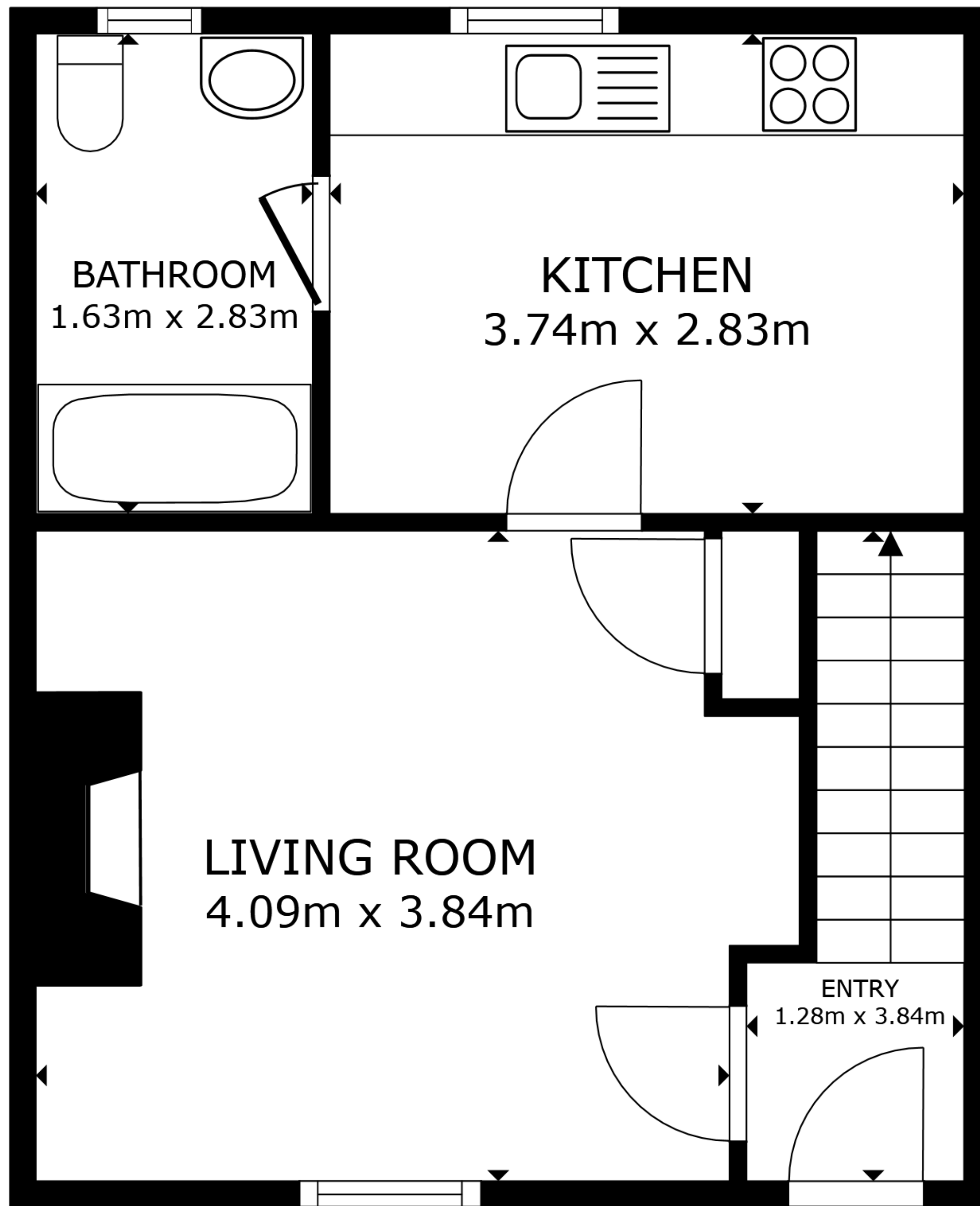
FLOOR 1
