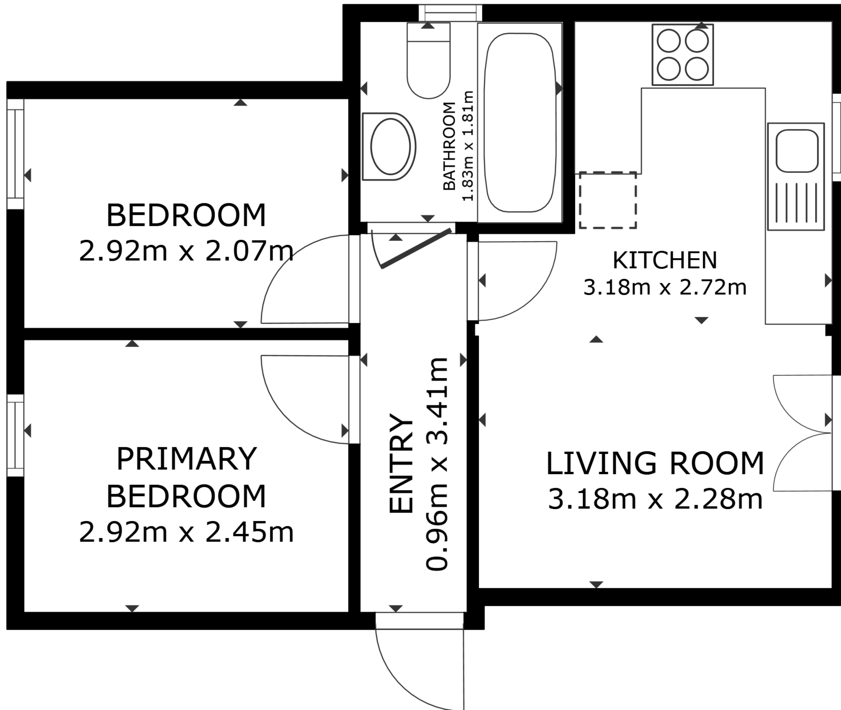
FLOOR PLAN
