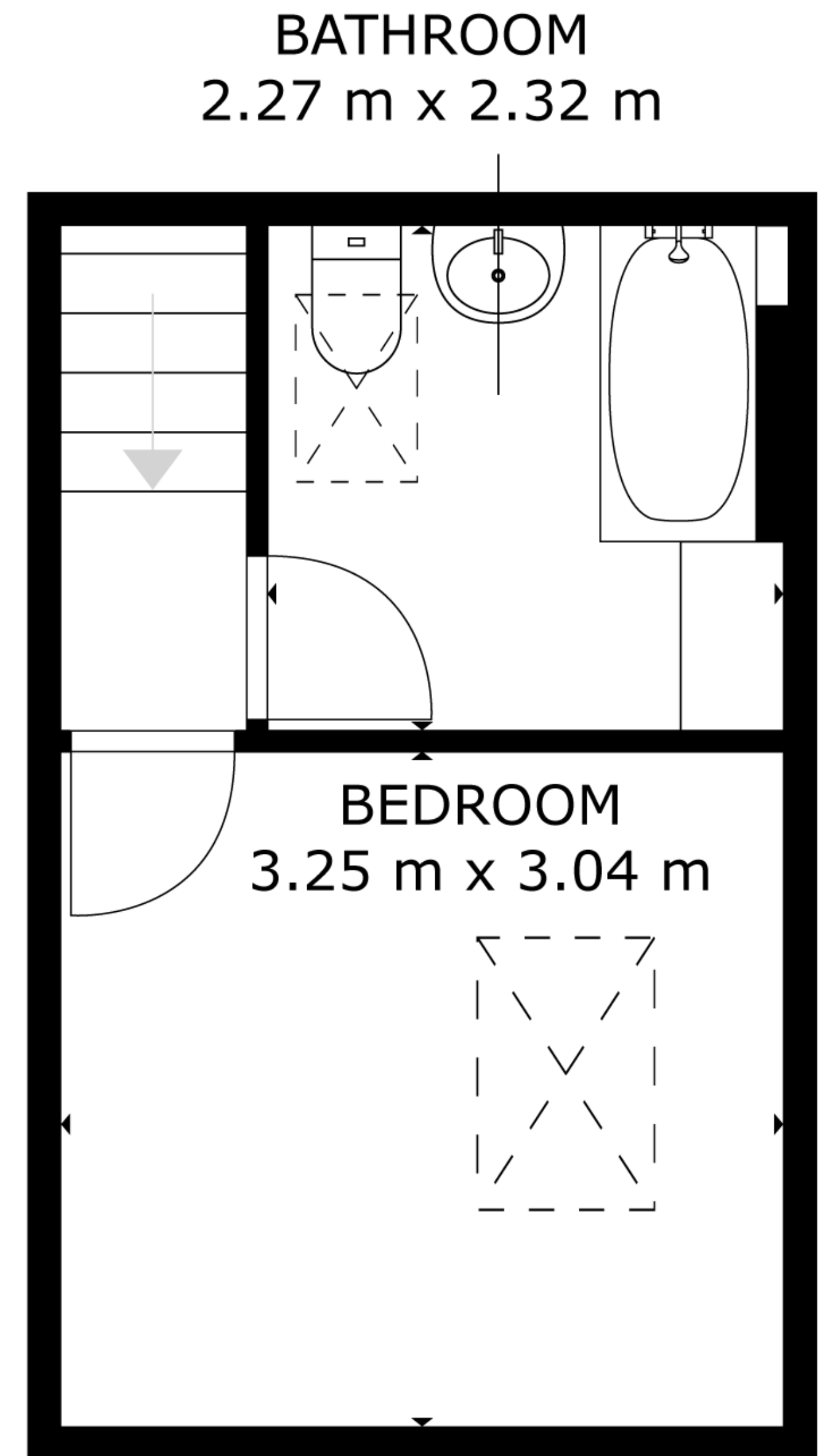
FLOOR 3
