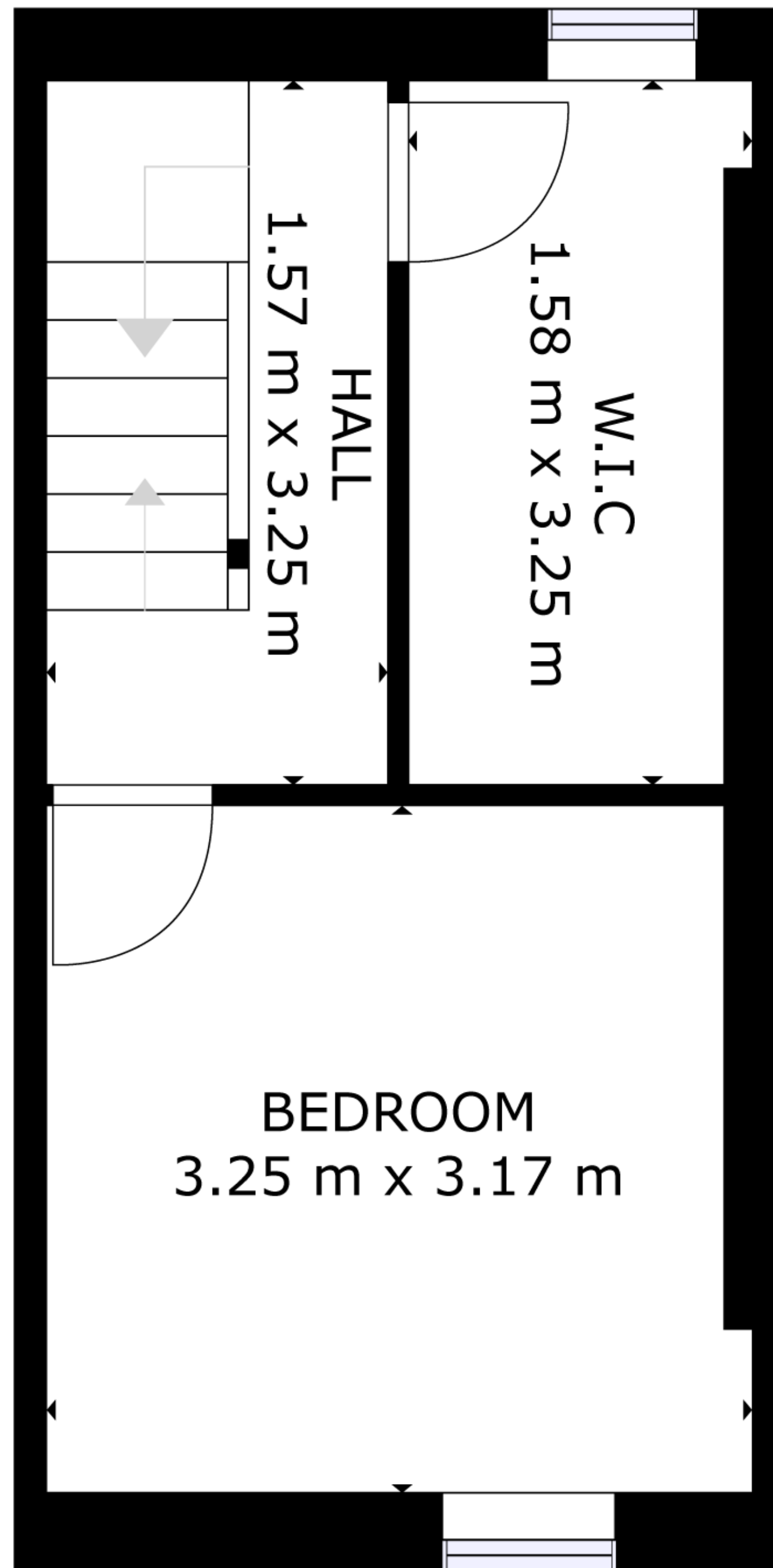
FLOOR 2
