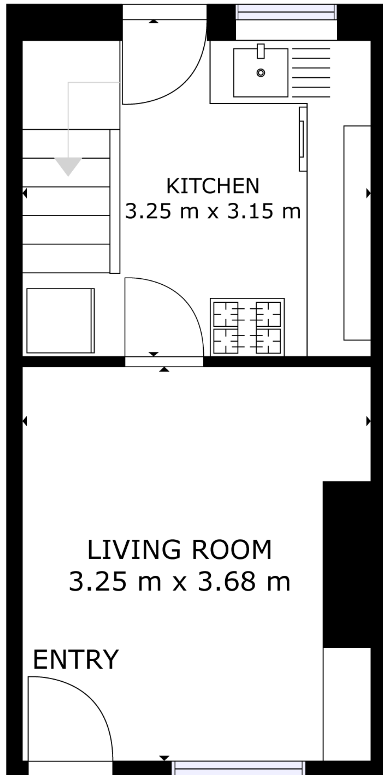
FLOOR 1
