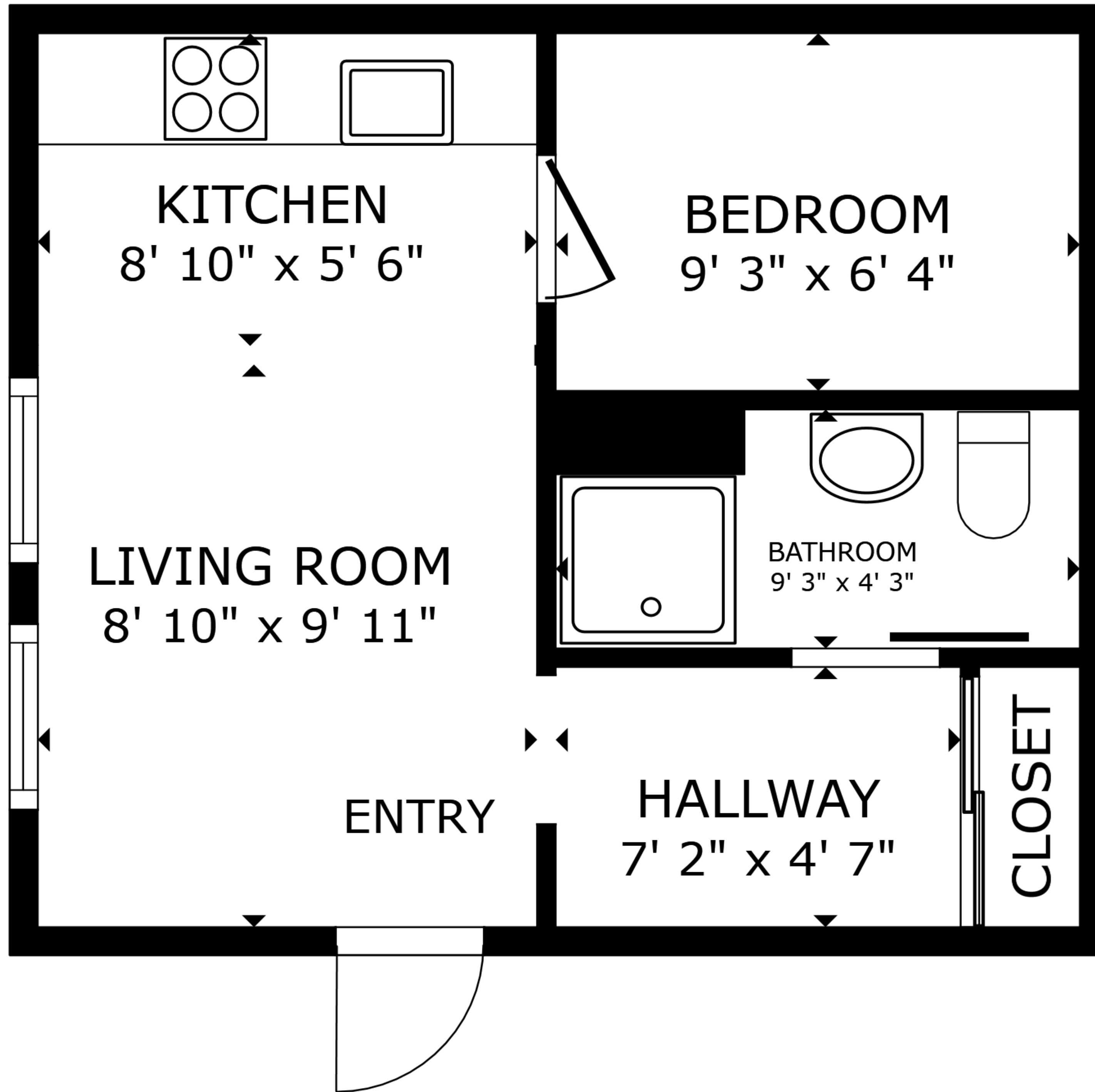
FLOOR PLAN
