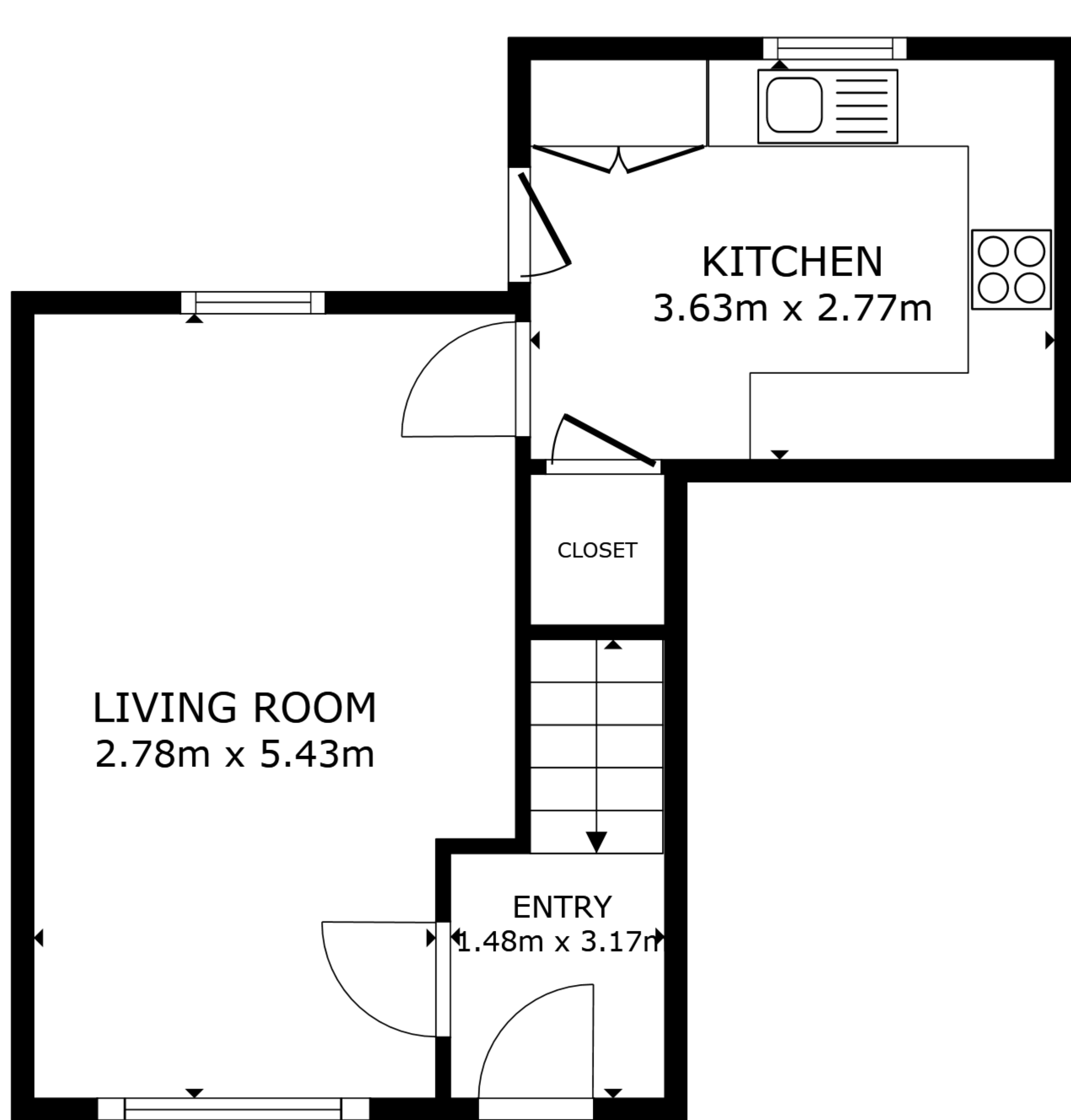
FLOOR 1
