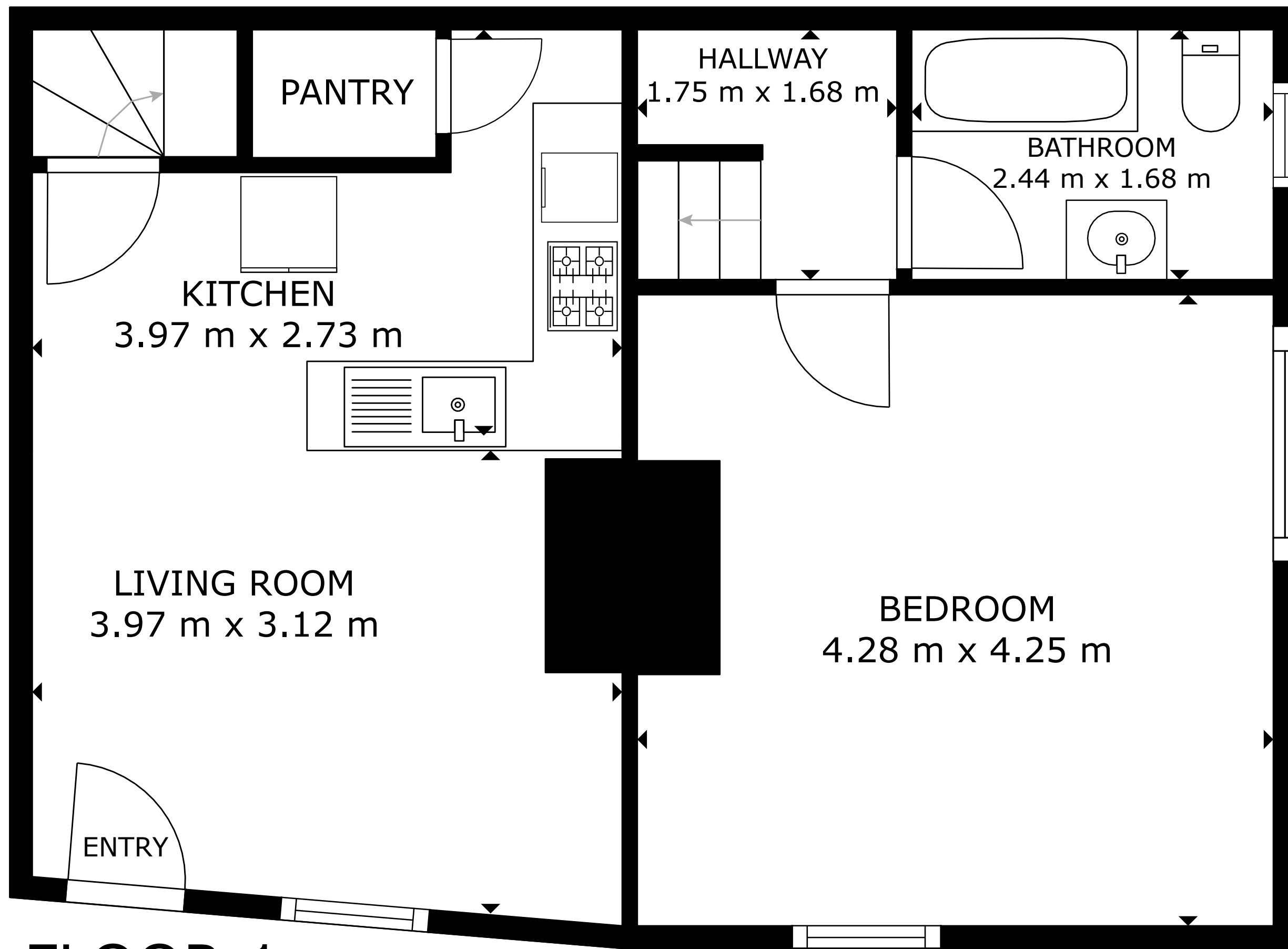
FLOOR 1
