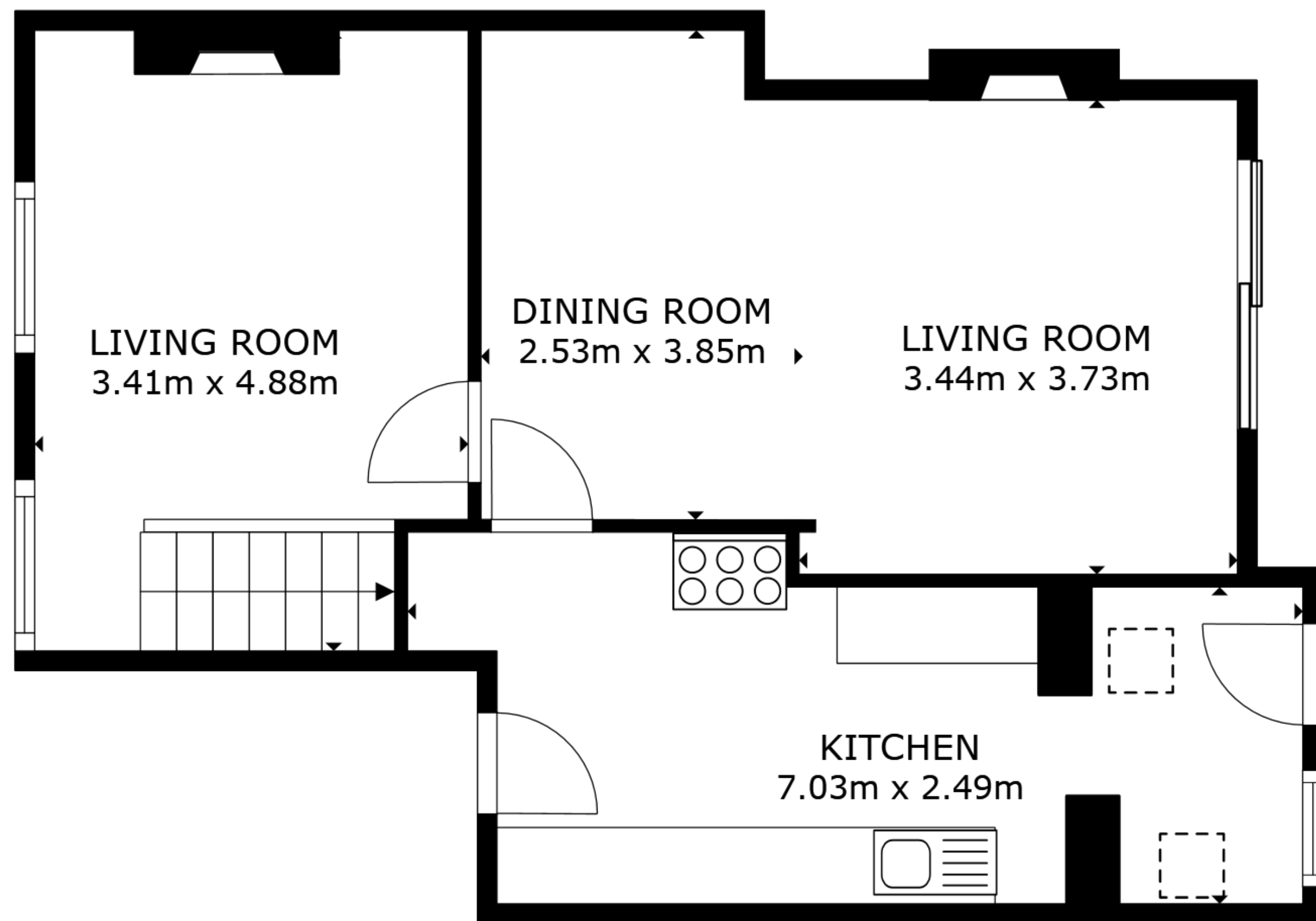
FLOOR 1
