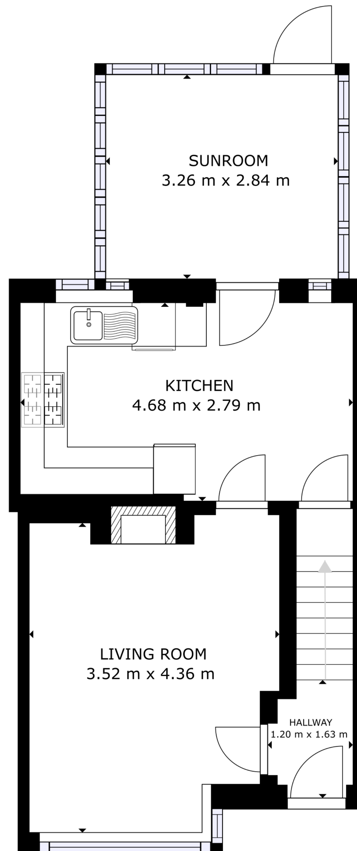
FLOOR 1
